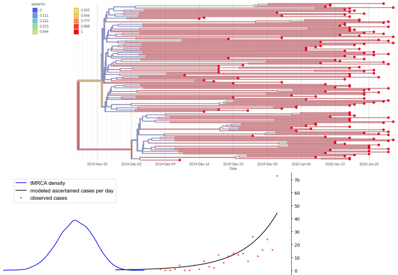
Figure 5 - BEAST2 exponential growth HKY 0.0008/subs/site/year and likelihood of the onset curve (ESS > 300) link
