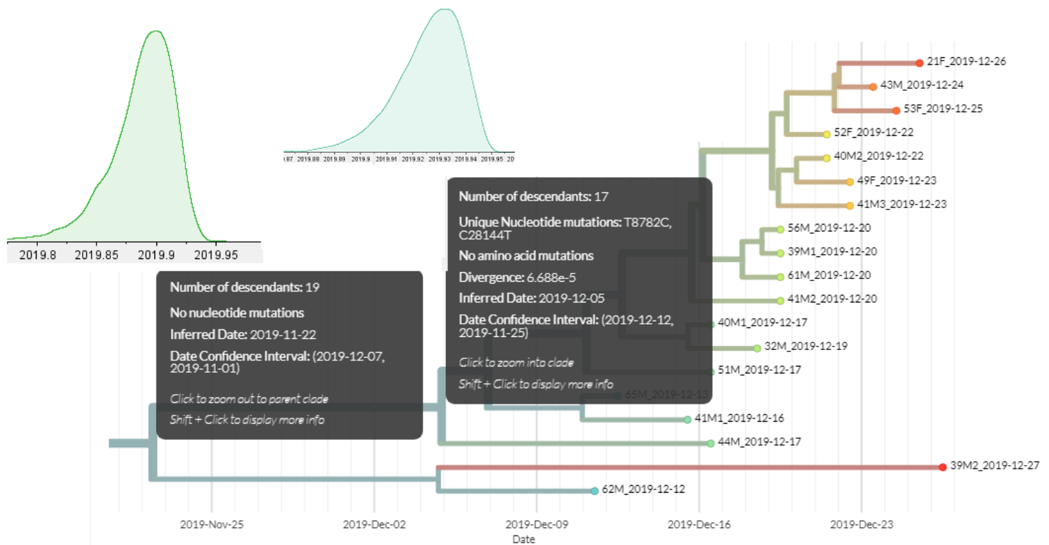
Figure 3 - BEAST skygrid HKY 0.0008 subs/site/year (ESS > 500) link
