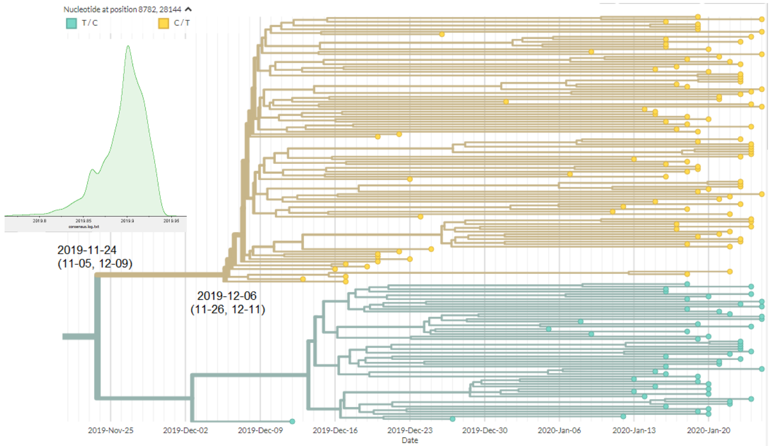
Figure 4 - BEAST skygrid (10) HKY 0.0008 subs/site/year (ESS > 200) link
