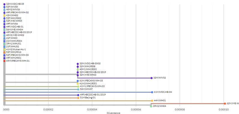
Figure 1 - Tree of the 37 genomes from 19 patients link
