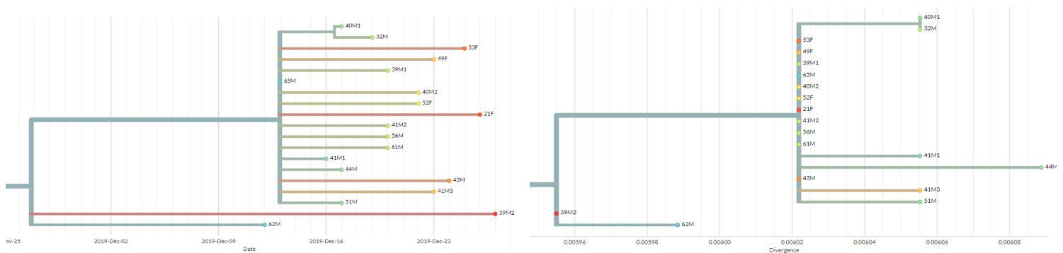
Figure 2 - Tree of the 19 consensus sequences obtained for each patient, dated with onset dates and rooted by adding the putative recombinant bat virus from [13a] link
