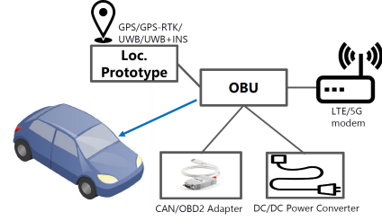
Fig. 4. Basic hardware components of the OBU.
