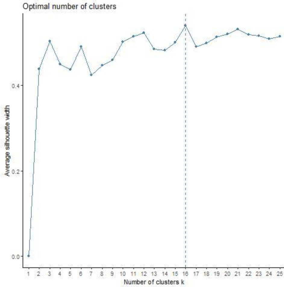
Supplementary figure 2. Silhouette plot for the mitochondrial DNA analysis, finding 16 optimal clusters.
