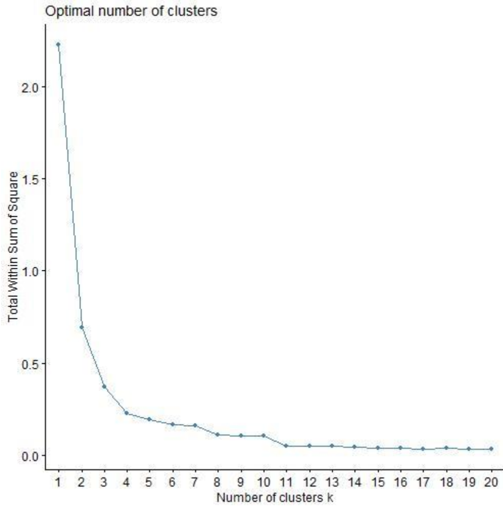
Supplementary Figure 1. Elbow plot for the Gene Content method, where an optimum of 12 clusters was found.
