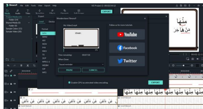
Gambar 6. Proses rendering
