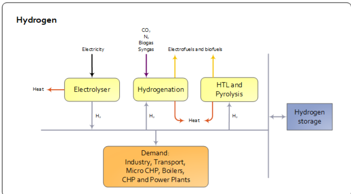
Illustration of components involved when the EnergyPLAN model calculates hourly balancing of the HYDROGEN system including interactions with other parts of the whole system.
