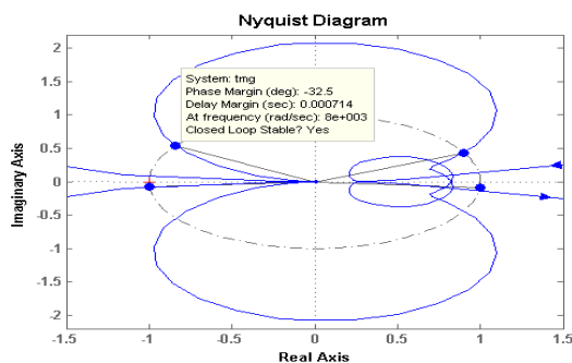
Figure 10. Nyquist plot of minor loop gain
