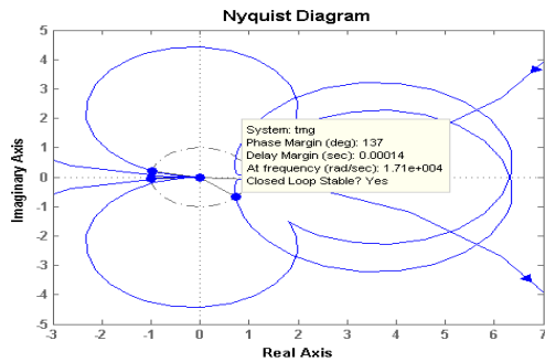
Figure 22. Nyquist plot of INV 1 & 5 are disconnected
