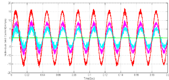
Figure 25. Individual grid current (Amp)
