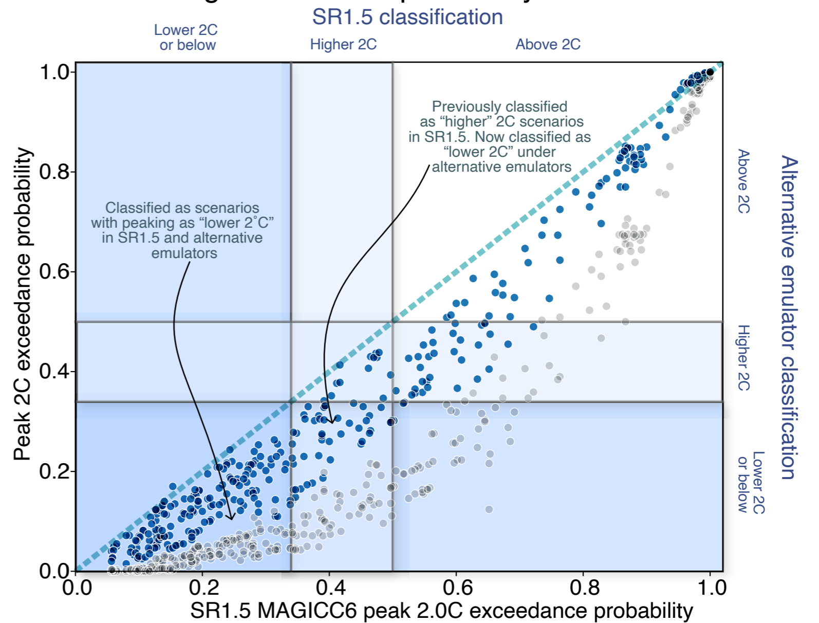
d Peaking exceedance probability of 2°C
