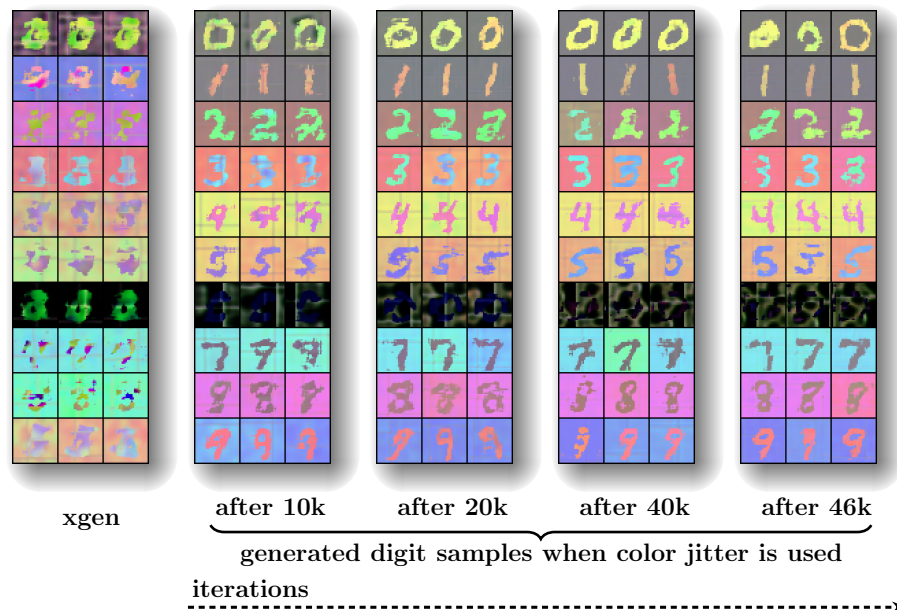
Figure 11. Double Colored MNIST samples obtained using addition of color jitter. We observe that it leads to generation of samples that are not indicative of the actual samples from the Double Colored MNIST dataset. We observe that there is difference between with/without augmentation in terms of the brightness, contrast, overall image representations. Specifically, digit 6 loses its shape, texture, colors. Similarly, digits 0,1 are generated using different colors in contrast to Fig. 10. Therefore, the visual samples indicate possibly why the classifier’s accuracy drops by around 10%.
