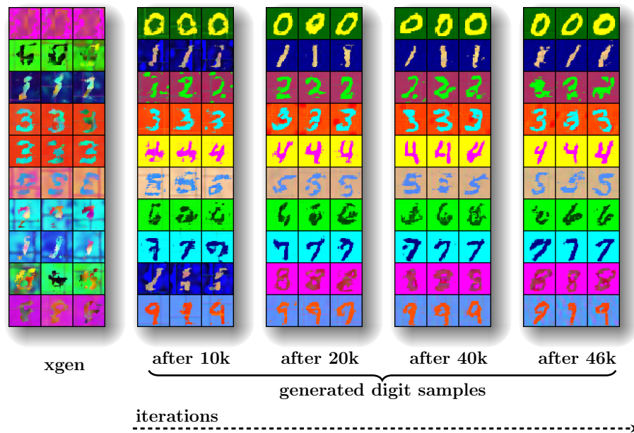
Figure 10. Double Colored MNIST samples obtained using default hyper-parameters mentioned in CGN [1].
