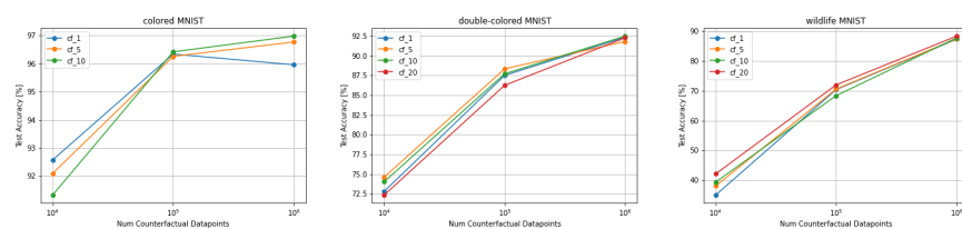
Figure 5. Recreated MNIST Ablation Study
