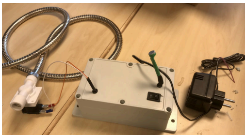
Figure 2. Hardware prototype
