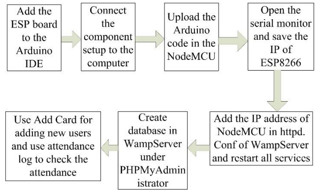
Fig. 7 Flow of the System implementation
