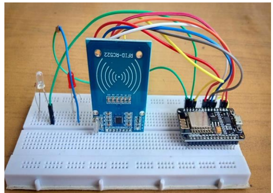
Fig. 5 Photograph of Diagonal view of the system
