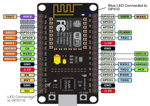
Fig. 2 Pin configuration of ESP8266 [10], [11]
