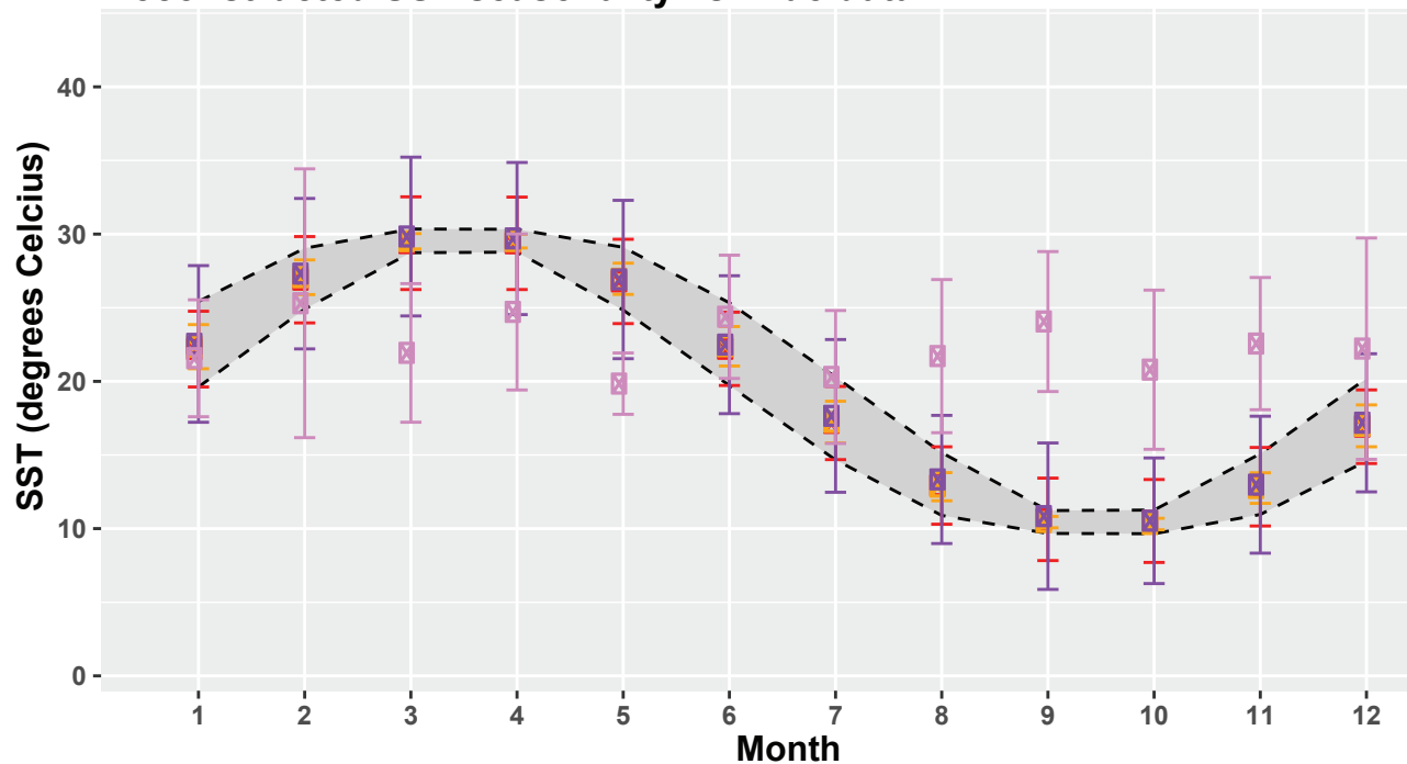
B Case 1, uneven sampling at 1.55 mm interval Reconstructed SST seasonality vs. True data
