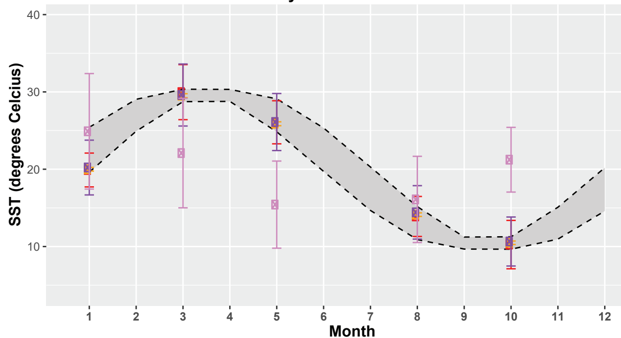
A Case 1, even sampling at 2 mm interval Reconstructed SST seasonality vs. True data
