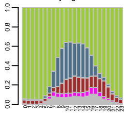
Survey age 55-64
