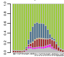
Survey females
