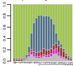
Synthetic age 55-64
