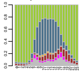
Synthetic males
