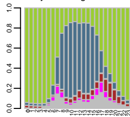
Synthetic age 25-54
