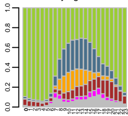
Survey age 18-24
