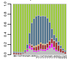
Synthetic all
