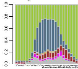
Synthetic females
