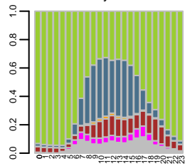
Survey males
