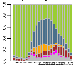
Synthetic age 18-24
