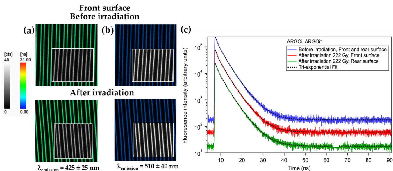
Figure 13. (a) Composite FLIM and fluorescence intensity microscopy images of the laser-induced structure ( 11 \text{ TW}/\text{cm}^2 ) before and after irradiation for an emission at 425 nm from the front surface; the color-code represents the mean lifetime obtained by FAST-FLIM algorithm (color scale from 0 to 31 ns); inset: luminescence intensity only (grey-scale from 0 to 45 counts). (b) Same composite FLIM and luminescence intensity images for an emission at 510 nm. (c) Luminescence decays in arbitrary units for the emission at 425 nm of the same structure before and after irradiation for the two surfaces, and fitting curves thereof using three exponential decay functions.
