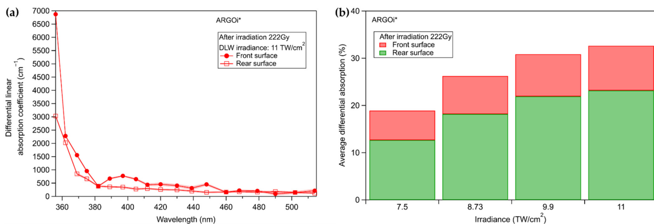
Figure 9. (a) Differential linear absorption coefficient of the laser-inscribed structures (11 TW/cm 2 ) for the two planes after irradiation at 222 Gy X-ray dose in the ARGOi* glass sample. (b) Average differential absorption of the inscribed structures for all DLW irradiance (as from Figure 9a).
