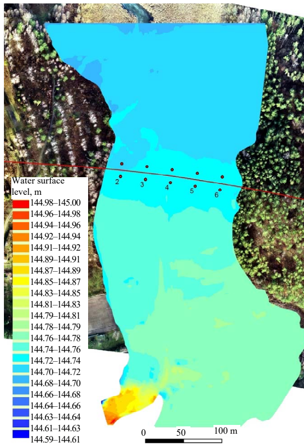
Fig. 5. Water surface level according to the results of modeling a breakthrough wave
