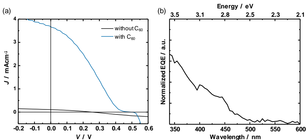
Figure 3. a) Photovoltaic characterization of fabricated TPV devices. J - V measurements under AM1.5G illumination for Zn(O,S) devices with S content x \approx 0.6 , with (blue) and without (gray) the organic C 60 ETL.
