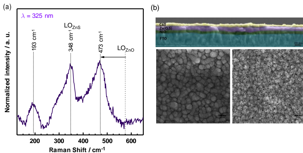
Figure 2. a) Raman spectrum of FTO/ZnO 1-x S x for relative sulfur content x = \frac{S}{S+O} = 0.6 acquired with 325 nm excitation wavelength. The main peaks observed are a characteristic Zn(O,S)-like mode at 193 cm -1 , the LO ZnS mode at 348 cm -1 , and the ZnO-like LO mode, shifted toward a lower Raman shift of 473 cm -1 . b) (top) CS-SEM pseudo-colored image of FTO/NiO/Zn(O,S)/C 60 . (bottom-left) Top-view SEM image of Zn(O,S) layer. (bottom-right) Top-view SEM image of C 60 film.
