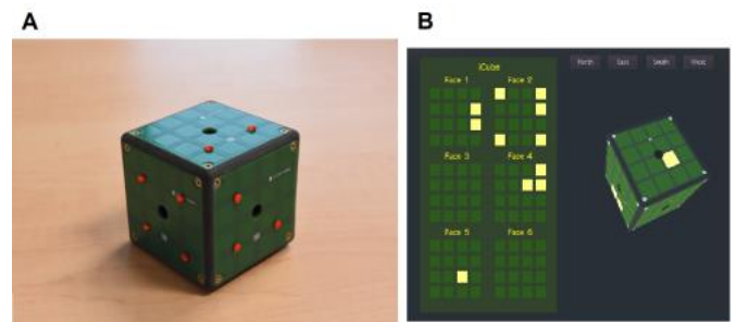
Fig. 1. The iCube. (a) Picture of iCube with raised pins positioned on its faces. (b) Example of real-time 3D rendering of iCube orientation with a snapshot of tactile sensors on each of the six faces. Yellow indicates cells currently touched.
