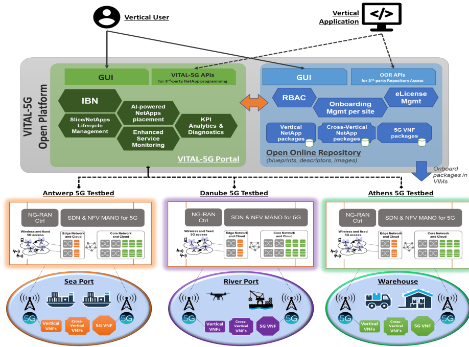
Figure 1: VITAL-5G architecture
