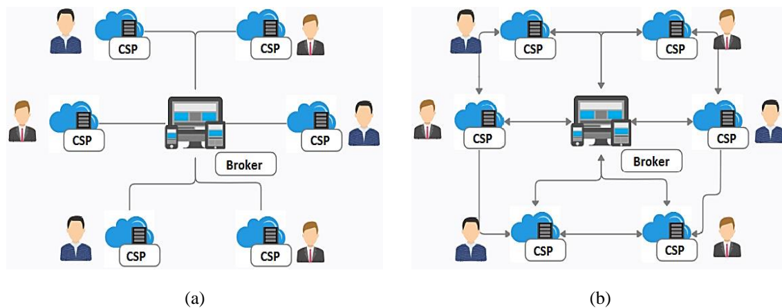
Figure 2. Architectures of monitoring in ICCE: (a) centralized and (b) decentralized
