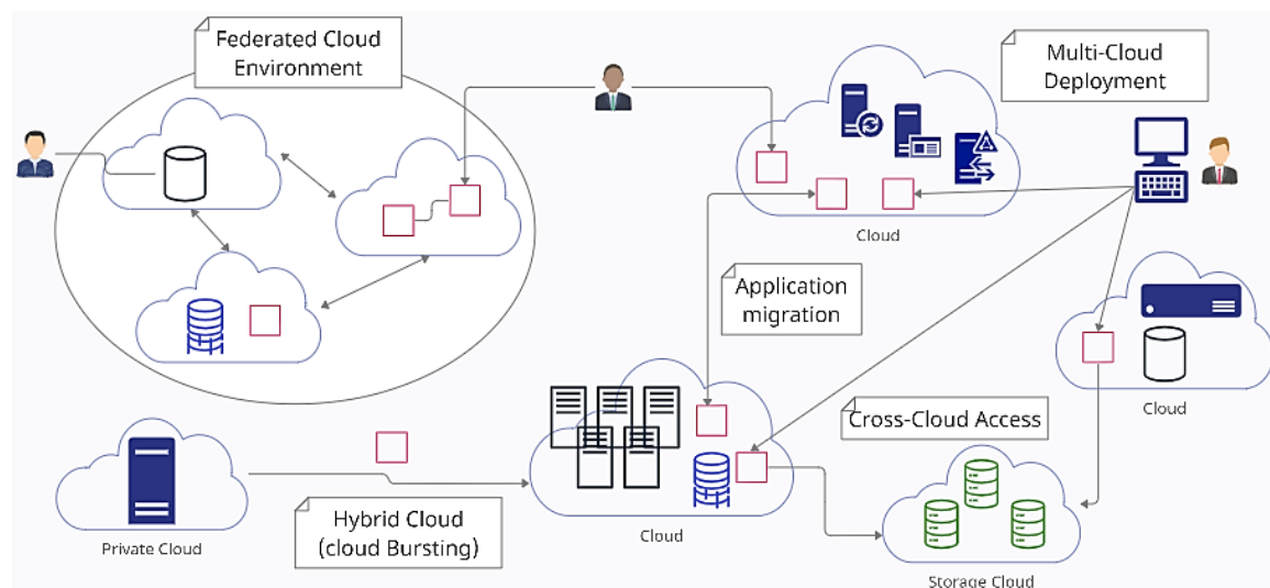
Figure 1. Scenarios and interoperability in the interconnected cloud computing environment
