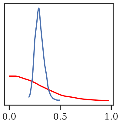
R0 hyperprior scale
