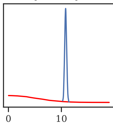
Output noise spread
