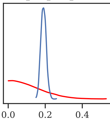
r_walk_noise_scale
