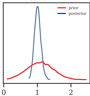
R0 hyperprior mean
