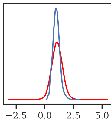
R0 prior
