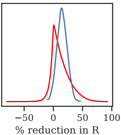
NPI effect (total)
