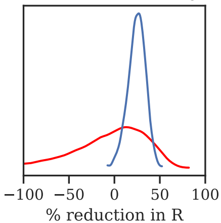
Mask effect (100% wearing)
