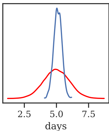
GI mean
