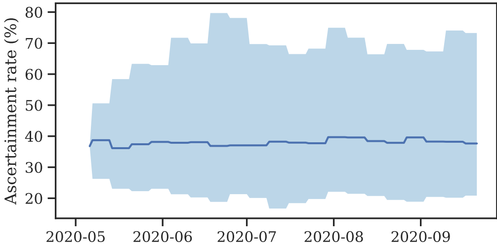
Simulated ascertainment rates over 100 runs
