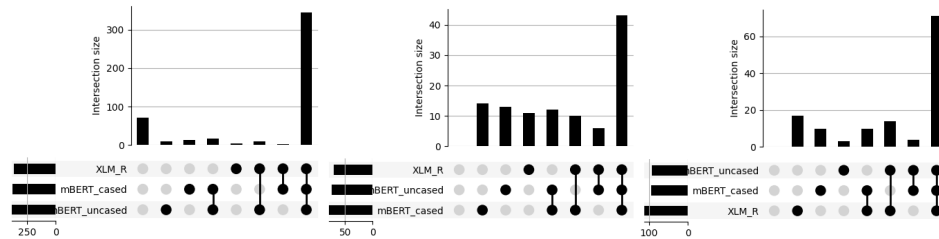
Fig. 3. Intersection of models predictions. Figures (a), (b), and (c) represent the true positive, false positive and false negative intersection sizes. The x-axis is interpreted as follows; from left to right, the first bar represents the number of instances that no system was able to find, the next three bars show the instances found by the respective individual models, the next three denote instances found by a pair of systems, while the last bar (the highest intersection) represents instances jointly found by all systems.
