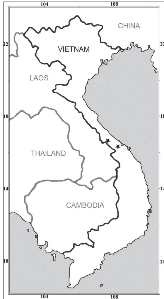
Figure 3. Distribution of Oreocharis phuongii sp. nov. from central Vietnam (shown by black stars).
