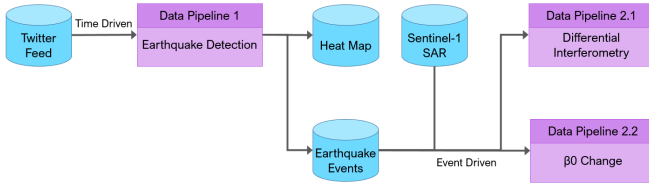
Fig. 3. Sequential Data Pipeline architecture.
