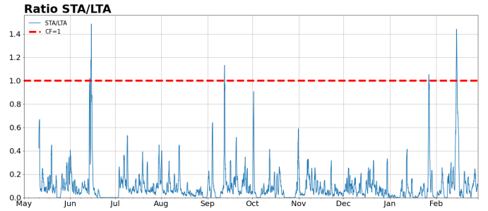
Fig. 4. The STA/LTA ratio of collected tweets from May 1, 2020 to March 1, 2021.
