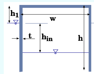
Fig. 4.37 – Schematic of a thin wall floating body.
