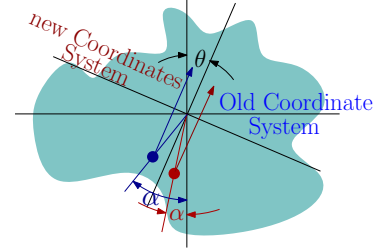
Fig. 4.46 – Arbitrary body rotates in \theta and the buoyancy centroid rotates in \alpha . The brown \alpha shows the case of stable scenario. The purple depicts the large \alpha not stable case.
