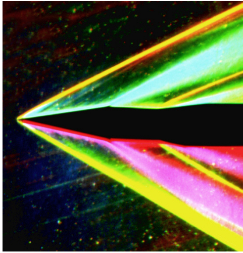
Fig. 15.9 – Color-schlieren image of a two dimensional flow over a wedge. The total deflection angle (two sides) is 20^\circ and upper and lower Mach angel are \sim 28^\circ and \sim 30^\circ , respectively. The image show the end-effects as it has thick (not sharp transition) compare to shock over a cone. The image was taken by Dr. Gary Settles at Gas Dynamics laboratory, Penn State University.
