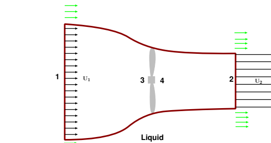
Fig. 6.4 – Propeller schematic to explain the change of momentum due to velocity.
