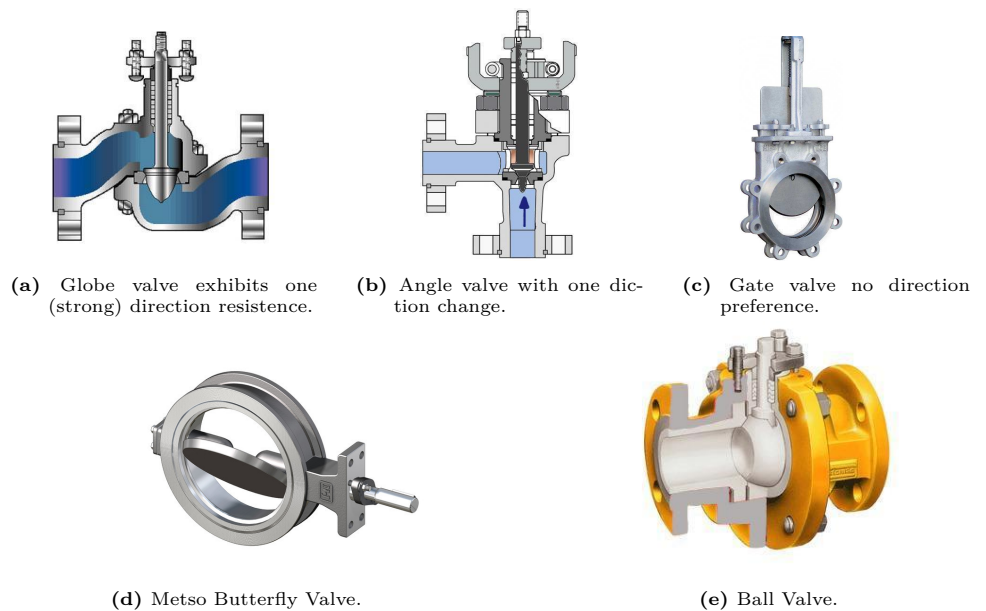
Fig. 11.13 – Possible “switches” valves of pipe network are exhibit. The various design of valve creates different resistance for the switching and regulation. The gate valve is typically design to on or off mode (an improved design is a ball valve) while the other two are used in addition for regulation (flow control). Clearly, the resistance in the gate valve is less because there is change in the flow direction. The Figures 11.13d and 11.13e represent additional design of no change of flow direction.
