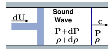
Fig. 14.1 – A very slow moving piston in a still gas.
