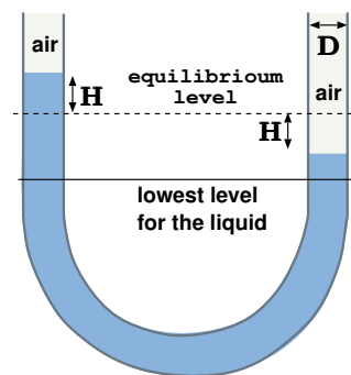
Fig. 7.5 – Flow in an oscillating manometer.
