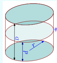
Fig. 4.57 – Upright floating cylinder.
