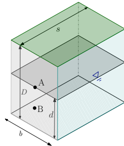
Fig. 4.47 – Rectangular body floating in a liquid for stability analysis.
