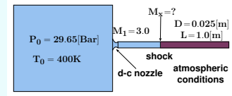
Fig. 14.22 – The schematic of Example (14.19).
