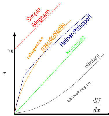
Fig. 1.5 – The different of power fluids families.
