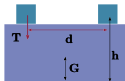
Fig. 4.59 – Measurement of GM of floating body. M_{weight} = T d (4.165)
