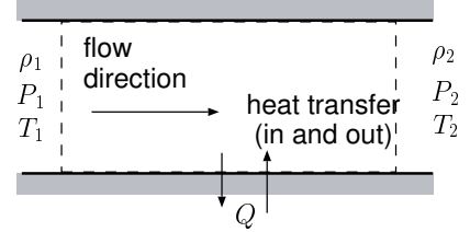
Fig. 14.39 – The control volume of Rayleigh Flow.
