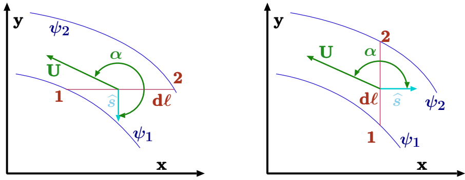
(a) Streamlines with element in X direction. (b) Streamlines with straight in Y direction.
