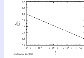
Fig. 3.13 – The ratio of the moment of inertia of two-dimensional to three-dimensional.
