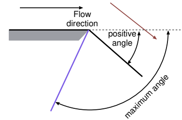
Fig. 15.21 – The definition of the angle for the Prandtl–Meyer function.
