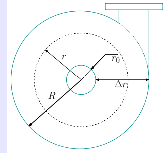
Fig. 5.15 – schematic of single stage centrifugal pump.
