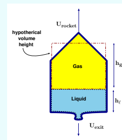
Fig. 6.12 – Nozzle schematics water rocket for the discussion on the forces for example 6.8
