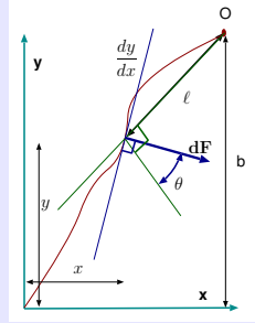
Fig. 4.33 – The difference between the slope and the direction angle.
