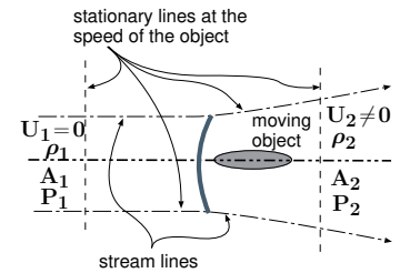
Fig. 14.15 – The diagram that reexplains the shock drag effect of a moving shock.
