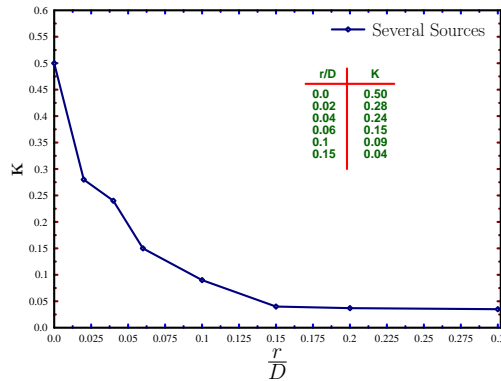
(e) diagram showing the resistance as function of the radius.
