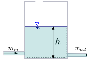
Fig. 5.6 – Height of the liquid for example 5.4.
