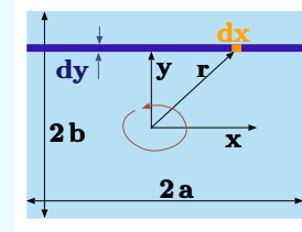
Fig. 3.14 – Rectangular Moment of inertia.
