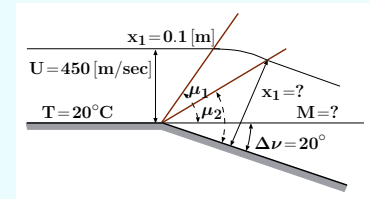
Fig. 15.29 – Schematic for Example 15.16.
