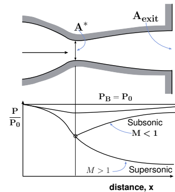
Fig. 14.4 – Flow of a compressible substance (gas) through a converging–diverging nozzle.
