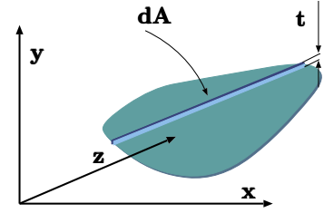
Fig. 3.3 – Thin body center of mass/area schematic.
