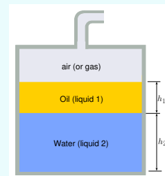
Fig. 1.15 – Two liquid layers under pressure.
