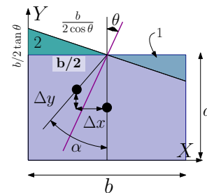
Fig. 4.44 – The Change Of Angle Due Tilting.
