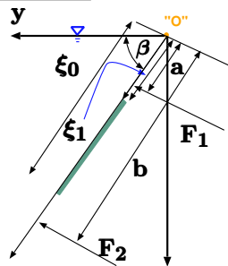
Fig. 4.22 – The general forces acting on submerged area.
