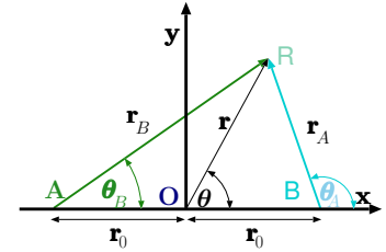
Fig. 12.10 – Combination of the Source and Sink located at a distance r_0 from the origin on the x coordinate. The source is on the right.
