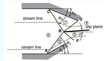
Fig. 15.18 – Illustration for Example (15.14).
