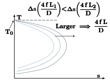
Fig. 14.23 – The effects of increase of \frac{4fL}{D} on the Fanno line.
