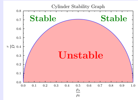
Fig. 4.52 – Cylinder in upright position stability line.
