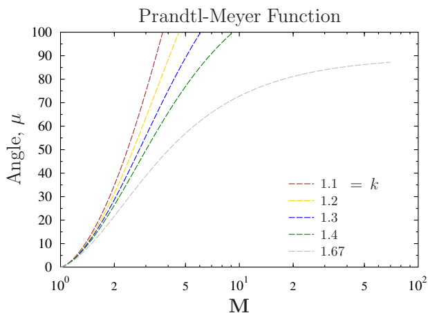
Fig. 15.26 – The angle as a function of the Mach number and specific heat.
