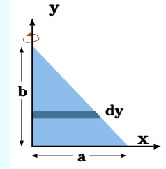
Fig. 3.16 – Triangle for example 3.11.
