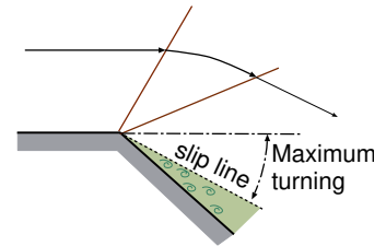
(15.95) Fig. 15.25 - Expansion of Prandtl-Meyer function when it exceeds the maximum angle.
