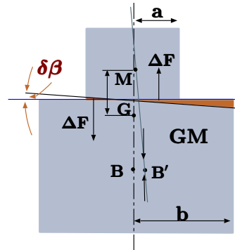
Fig. 4.60 – Calculations of GM for abrupt shape body.
