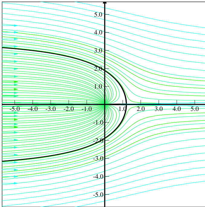
Fig. 12.20 – Uniform flow with a sink.
