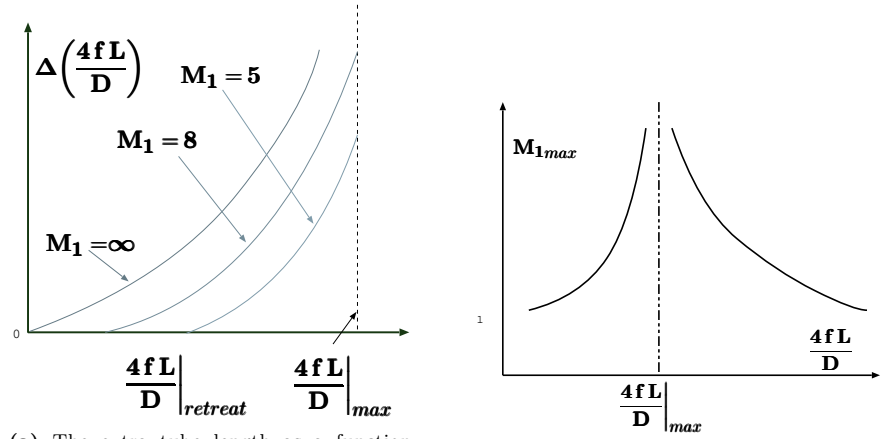
(b) The maximum entrance Mach number, M_{1max} to the tube as a function of \frac{4fL}{D} supersonic branch.
