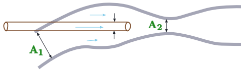
Fig. 5.13 – Water jet Pump.
