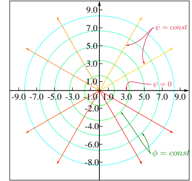
Fig. 12.7 – Streamlines and Potential lines due to Source or sink.
