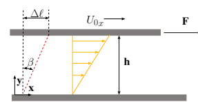
Fig. 1.3 – Schematics to describe the shear stress in fluid mechanics.
