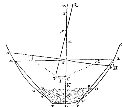
Fig. 4.41 – Bouguer Showing Metacenter.
