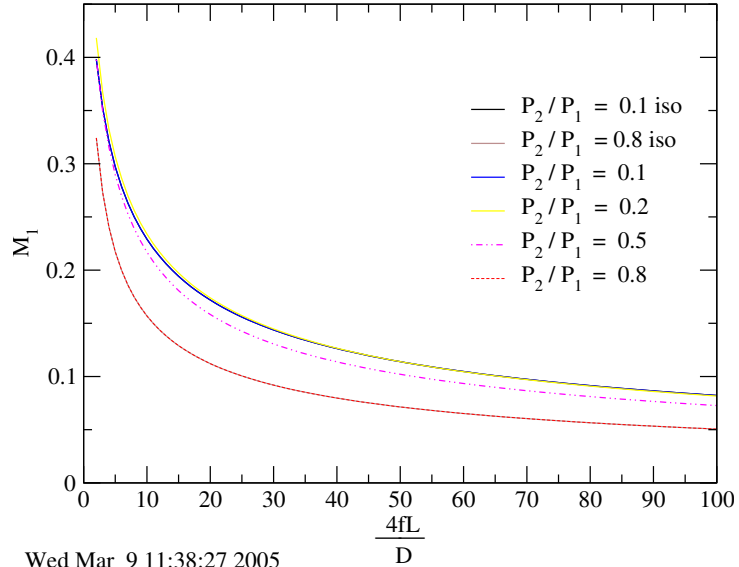
Fig. 14.38 – The entrance Mach number as a function of dimensionless resistance and comparison with Isothermal Flow.
