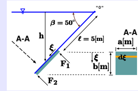
Fig. 4.20 – Rectangular area under pressure.
