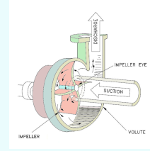
Fig. 5.14 – Schematic for a centrifugal pump. to be replaced
