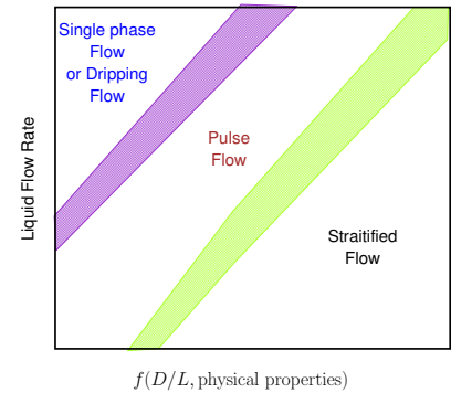
Fig. 16.14 – A flow map to explain the horizontal counter-current flow.
