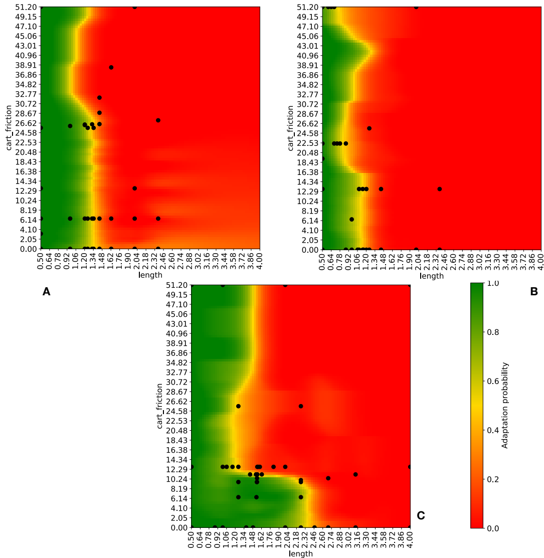
Figure 6: Adaptation probability heatmaps for PPO, SAC and DQN in the CartPole 2 environment
