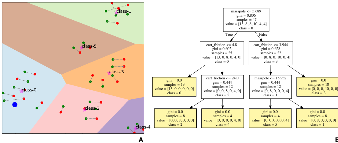
Figure 8: Visualization of frontier pairs found by ALPHATEST in the Cartpole 3 environment for PPO and their classification by means of a decision tree
