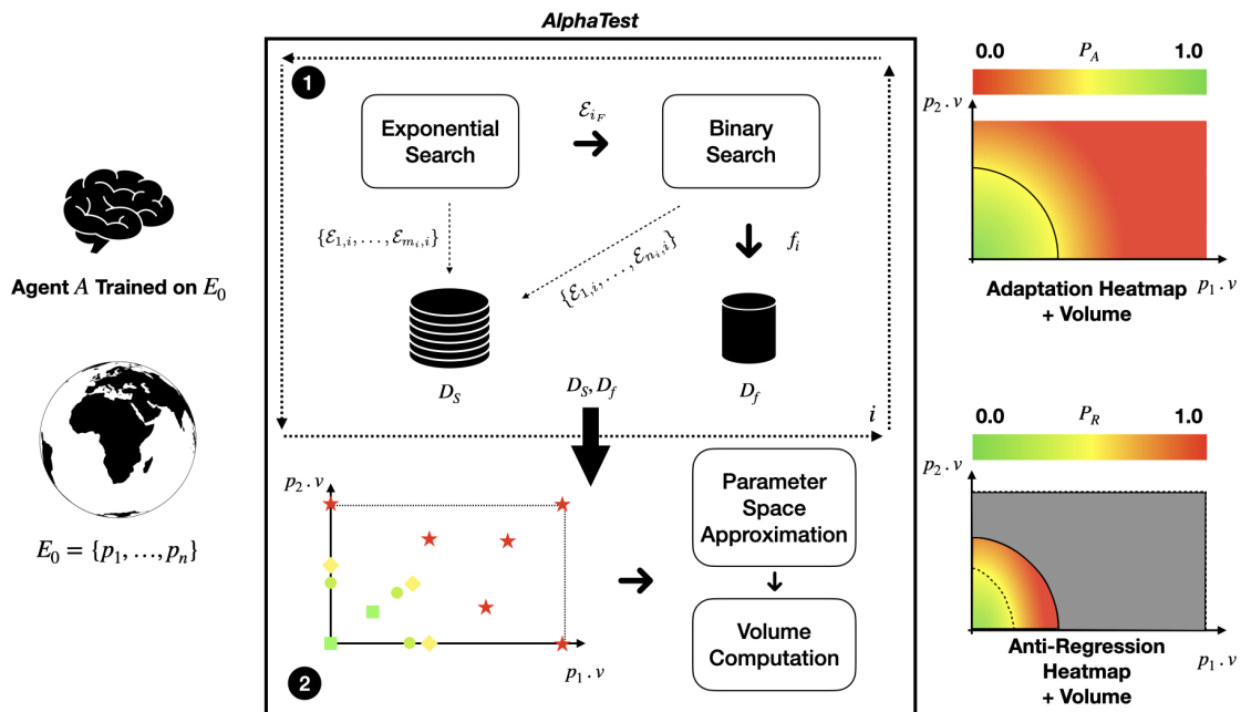
Figure 1: Overview of the approach implemented in ALPHATEST
