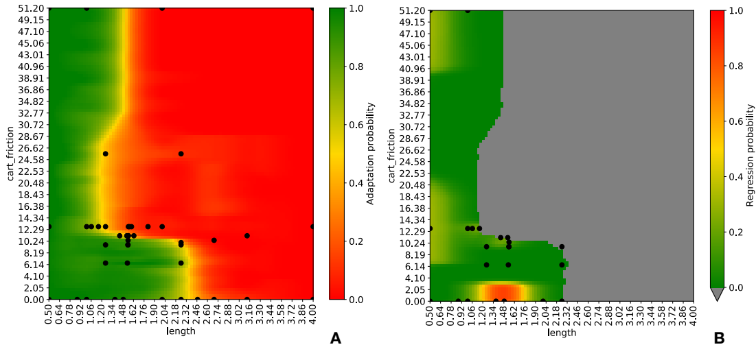
Figure 7: Adaptation and anti-regression probability heatmaps for DQN algorithm in the CartPole 2 environment
