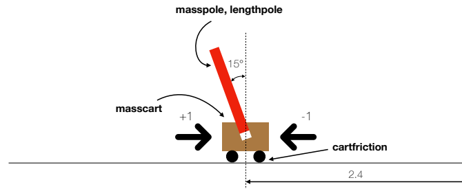
Figure 2: Representation of the Cartpole environment [6, 54], described by Barto et al. [5]
