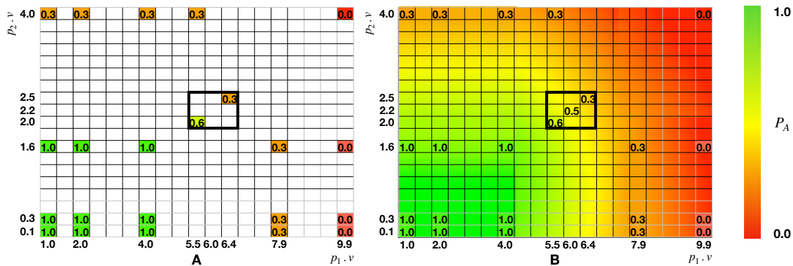
Figure 4: Adaptation probability heatmaps
