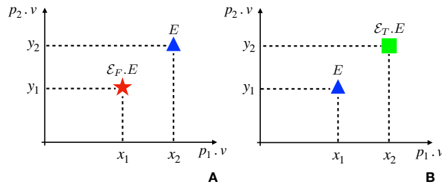
Figure 3: Environment dominance in two dimensions; E is the environment under analysis
