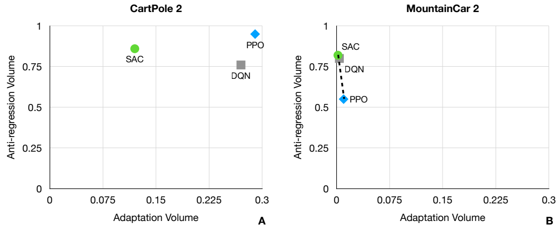
Figure 5: Trade-off between adaptation and anti-regression volumes
