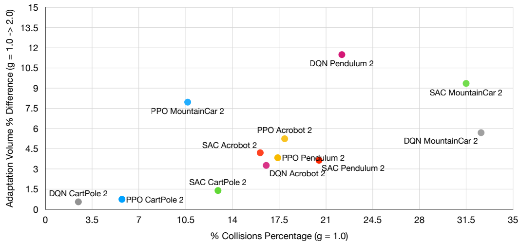
Figure 9: Relation between collisions percentage and adaptation volume percentage difference
