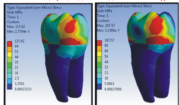
Figure 4: Von-Mises Stress distribution on restoration when tooth restored with Cention N at (a) 450 N and (b) 600 N Load was applied.
