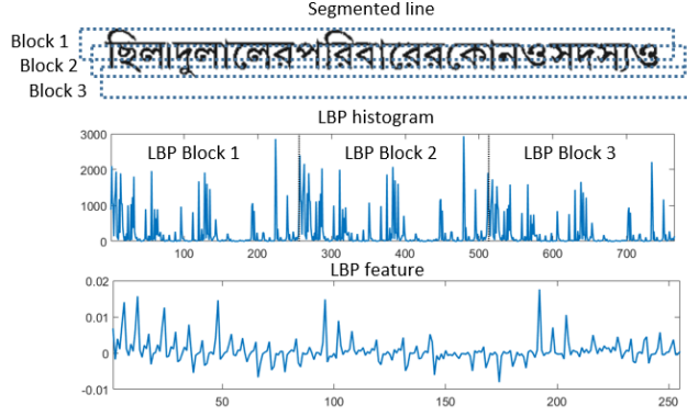
Fig 5. LBP features for script identification
