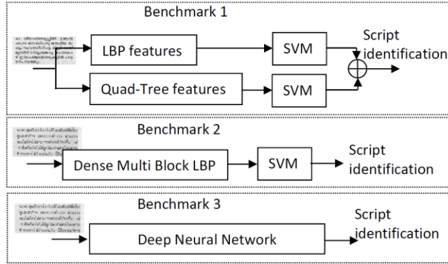
Fig 8. Benchmarks constructed in the paper
