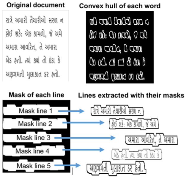
Fig 4 Line detection procedure
