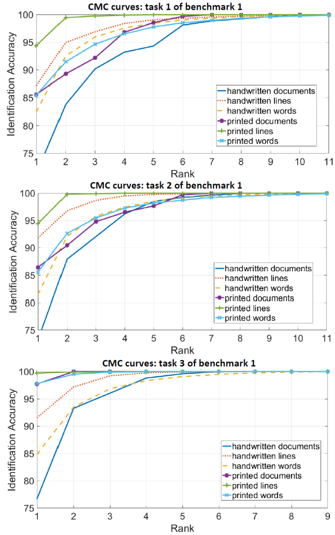
Fig 9 CMC curves of the three tasks of Benchmark 1. These CMC curves correspond to the results in bold in Table 5.
