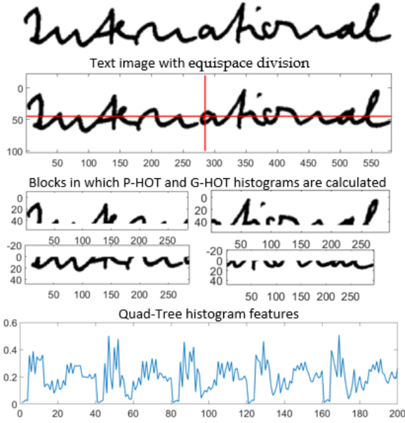
Fig 6. Quad-Tree Histogram for script identification
