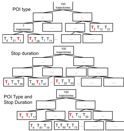
Figure 4: A sample set of single- and multiple-aspect trees that constitute the multiple-aspect forest.
