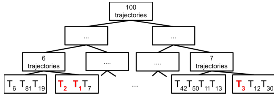
Figure 3: A sample single-aspect tree created using hierarchical partitioning.
