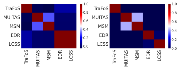
Figure 6: Pairwise agreement scores (Adjusted Rand Index) of the clustering schemes (Single linkage-left, Average linkage-right) using the different similarity metrics.
