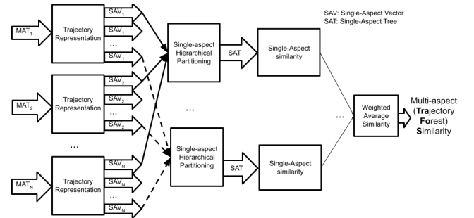
Figure 2: The steps of TraFoS similarity for MATs.
