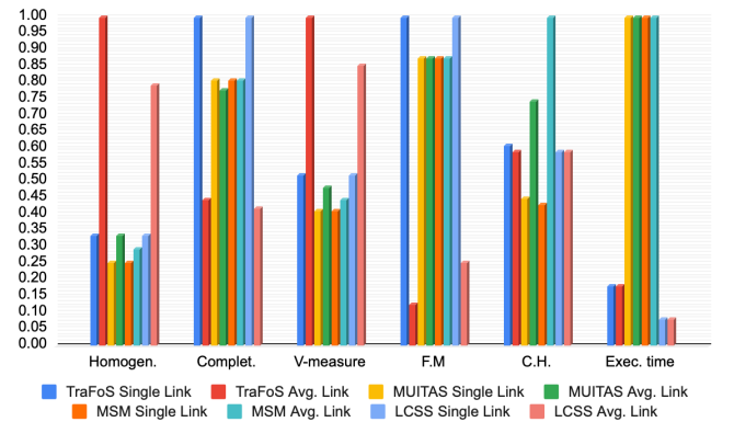
Figure 5: Summarizing evaluation results and execution time.
