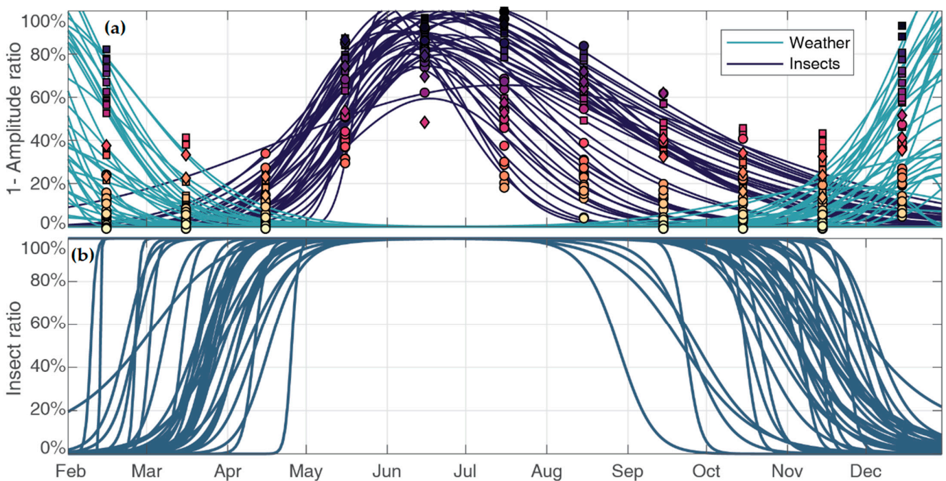
Figure 5. The insect-like signal (i.e., 1-amplitude ratio) is separated into insect and weather. (a) The sum of two skew-normal density functions representing insects (black) and weather (grey) is fitted for each radar (circle for France, square for German, and diamond for Benelux). (b) The proportion of insects in the original insect-like signal is estimated from the fitted density distribution functions of Figure 5a.
