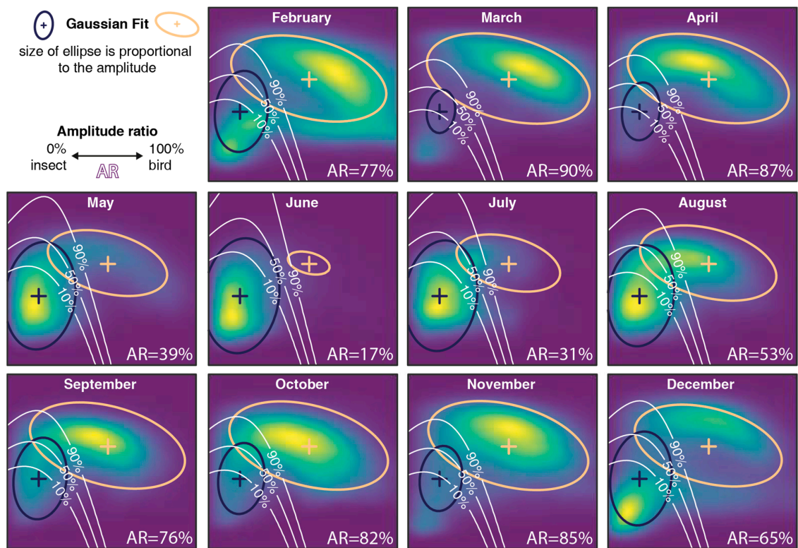
Figure 2. Monthly joint probability density function of airspeed and radial velocity standard deviation for the empirical (color-scaled surface) and fitted Gaussian distributions of birds (red lines) and insects (purple lines). The white contour line depicts the mapping of the proportion of birds and insects resulting from the fitted model. The x - and y -axis unit and range are the same as those in Figure 1, but the color-scale is normalized each month.
