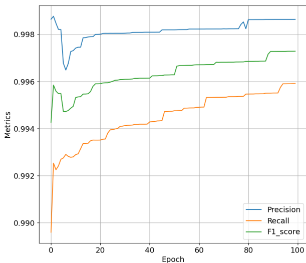
FIGURE 14: Comparison of performance metrics for stage 1 of architecture V over 100 epochs
