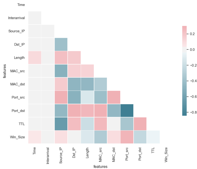
FIGURE 3: Correlation between IoT traffic features of Dataset 1
