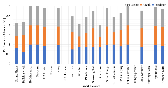
FIGURE 10: Performance comparison per device for architecture V
