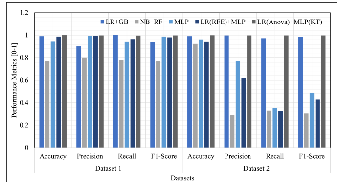
FIGURE 8: Performance comparison at stage 1
