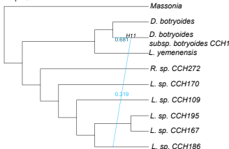
Rep 10 - network 1
