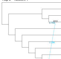
Rep 9 - network 1
