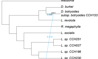
Rep 6 - network 2
