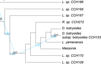
Rep 10 - network 2
