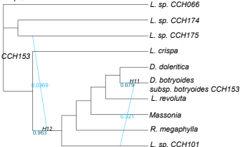
Rep 5 - network 2
