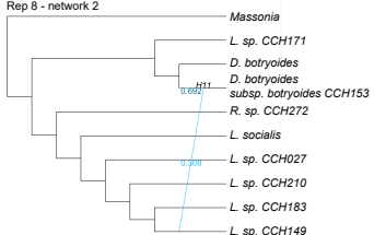
Rep 8 - network 2
