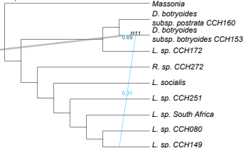
Rep 2 - network 2
