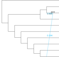
Rep 1 - network 1
