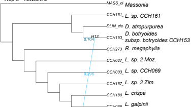
Rep 9 - network 2
