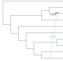
Rep 6 - network 1
