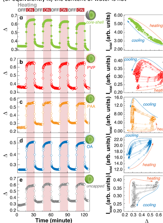
Figure 4. Evolution of the thermometric parameter ( \Delta ) in four thermal cycles for (a) core-shell, (b) PVP-capped, (c) PAA-capped, (d) OA-capped nanoparticles, and (e) uncapped nanoparticles. The corresponding dependence of the total integrated intensities ( I_{\text{total}} ) with \Delta are presented in f-j in consecutive heating-cooling cycles.
