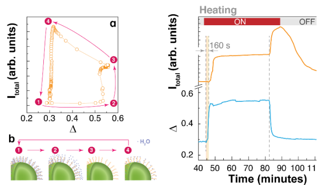
Figure 5. Water adsorption-desorption model exemplified for PAA-capped nanoparticles (a) Thermal hysteresis loop (second cycle) identifying four critical points. (b) Schematic representation of the water (blue dots) adsorption state in each of the critical points. In the initial state (1) the water content is maximum and the emission intensity is partially quenched. On state (2) water desorption from the PAA is thermally activated, producing the unquenching of the emissions. At state (3) the heating source is turned off; on cooling, the thermal quenching is reduced and the system reaches its maximum emission intensity on the state (4) when water re-adsorption occurs. (c) Time delay observed for the apparent enhancement during the initial heating cycle and the absence of such a delay when turning off the heating source.
