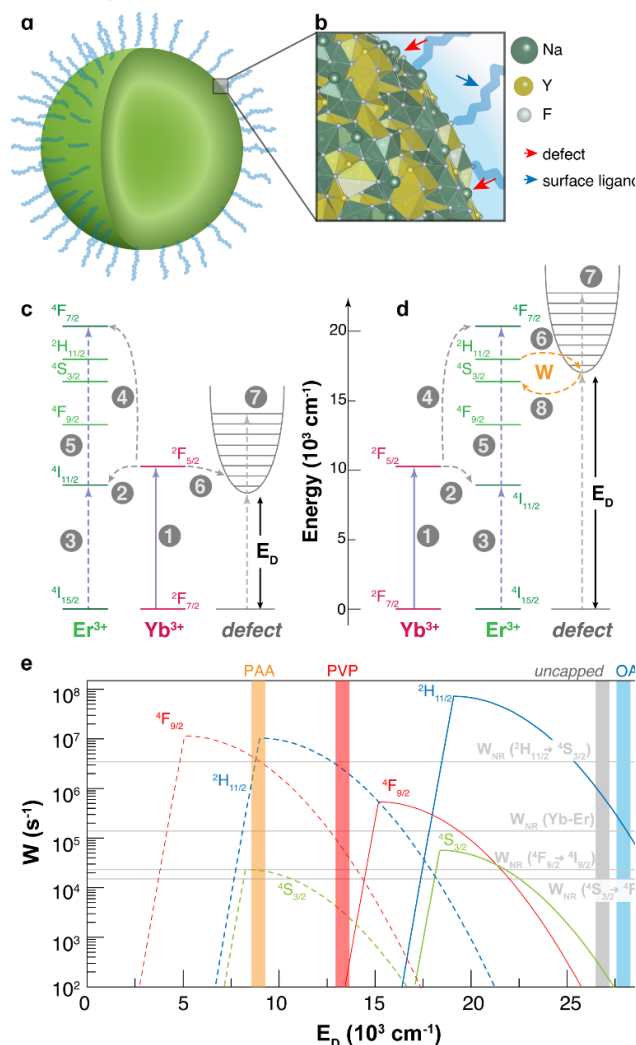
Figure 6. (a) Illustration of a \text{NaYF}_4 spherical nanoparticle and (b) its amplified image displaying surface defects and ligands. (c) and (d) are the two situations in which the defects would interact as energy donors. (1) is the \text{Yb}^{3+} absorption ( {}^2\text{F}_{7/2} \rightarrow {}^2\text{F}_{5/2} ); (2) and (3) are the first step in the Yb-Er UC process where the \text{Er}^{3+} ground population is excited to an
