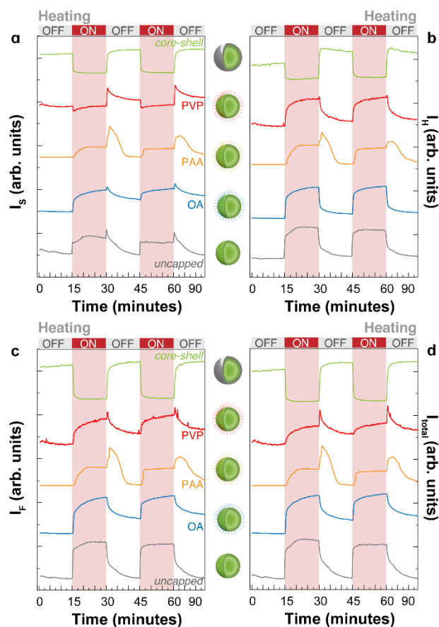
Figure 3. The integrated intensity in two thermal cycles corresponding to the (a) S transition ( I_S , ^4\text{S}_{3/2} \rightarrow ^4\text{I}_{15/2} ), (b) H transition ( I_H , ^2\text{H}_{11/2} \rightarrow ^4\text{I}_{15/2} ), (c) F transition ( I_F , ^4\text{F}_{9/2} \rightarrow ^4\text{I}_{15/2} ), and (d) the sum of the areas of S, H, and F transitions ( I_{\text{total}} ) for all the samples studied in this work.
