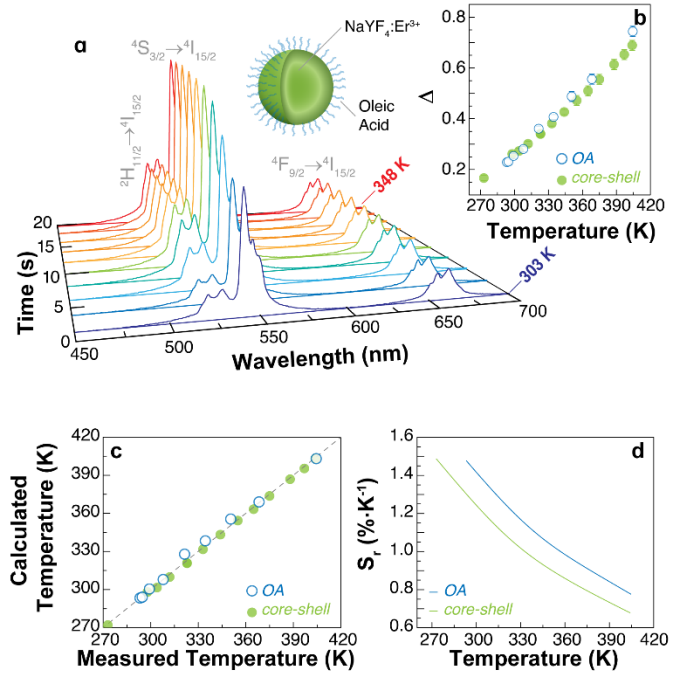
Figure 2. (a) Temperature dependence of the upconversion emission spectra of UCNPs-OA under 976 nm excitation ( \sim 30 W \cdot cm^{-2} ). The Er 3+ transitions are identified. (b) Calibration curve for the UCNPs-OA and core-shell NPs in the 293-405 K range. The calibration temperature is recorded using a Pt100 thermistor thermometer. (c) Comparison between the temperature values measured by the external thermometer ( x -axis) and those calculated using Eq. 2 ( y -axis) for the UCNPs-OA and core-shell NPs. The x=y line corresponds to the perfect agreement between both employed methods. (d) Relative thermal sensitivity of the thermometers in the calibration range.
