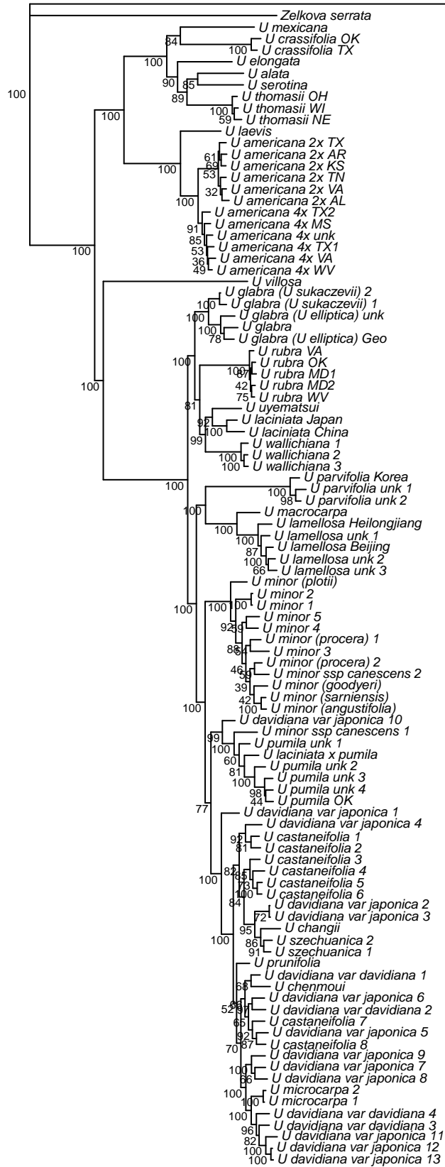
Figure S2. Concatenation phylogeny estimated by maximum likelihood, including tetraploids and putative hybrids, with strict filtering of loci to maximize power to detect and filter paralogs.
