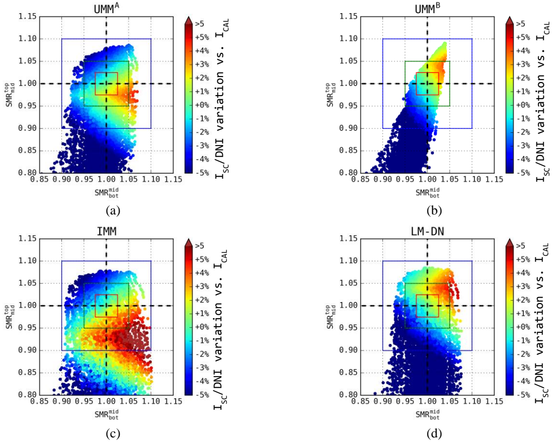
FIGURE 3. Spectral variations of the normalized current during 2014 in Madrid for the representative (a) UMM-A, (b) UMM-B, (c) IMM and (d) LM-DN multi-junction solar cells analyzed in this work.
