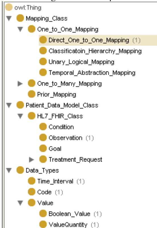
Figure 6.4.3. The mapping ontology of KDOM
