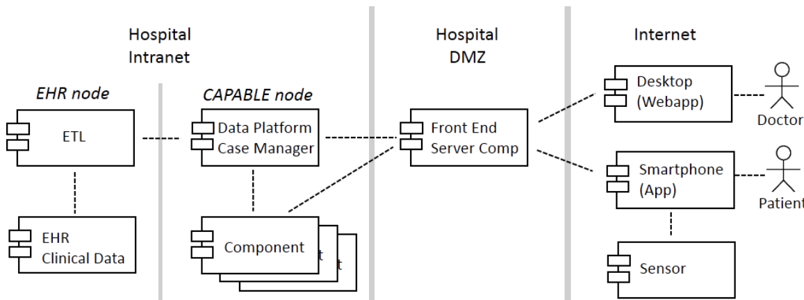
Figure 16.2.1. UML Component Diagram illustrating the Deployment Architecture envisioned for the CAPABLE system. This is a generic architecture that will be tailored to the specific requirements of the Hospital settings before starting the pilot trials.
