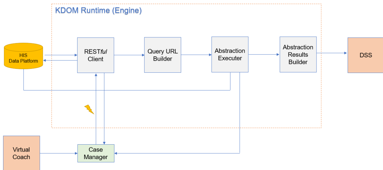
Figure 6.4.7. System Architecture Diagram
