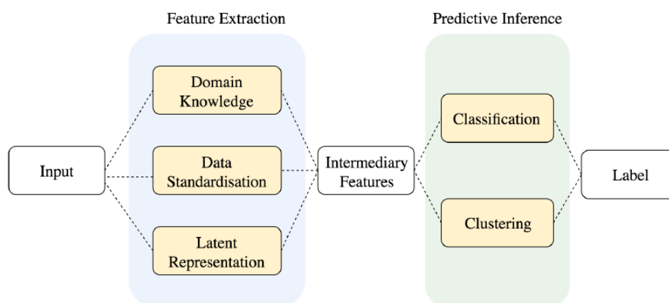
Figure 8.1. General Machine Learning Pipeline
