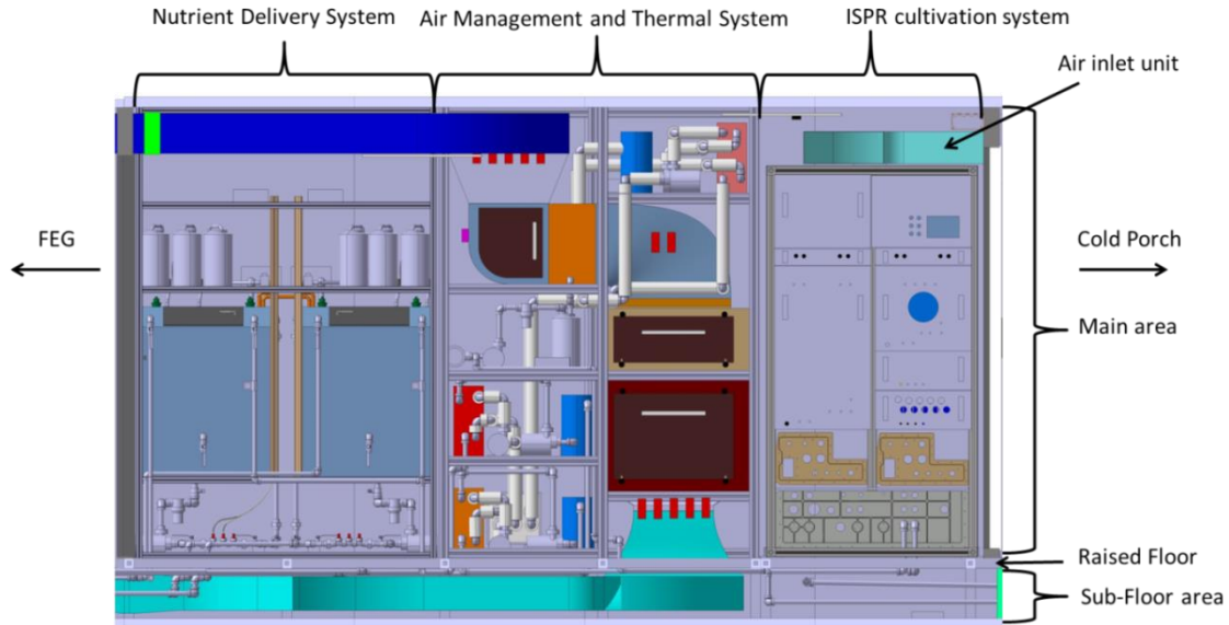
Figure 8. Service Section cut view – South side (Credit: DLR).
