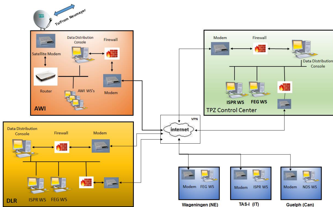
Figure 17. Layout of the EDEN ISS User Segment including the different workstations (WS) (Credit: Telespazio).
