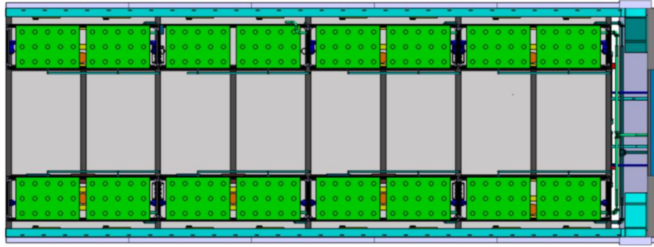
Figure 11. Future Exploration Greenhouse – Top view (Credit: DLR).
