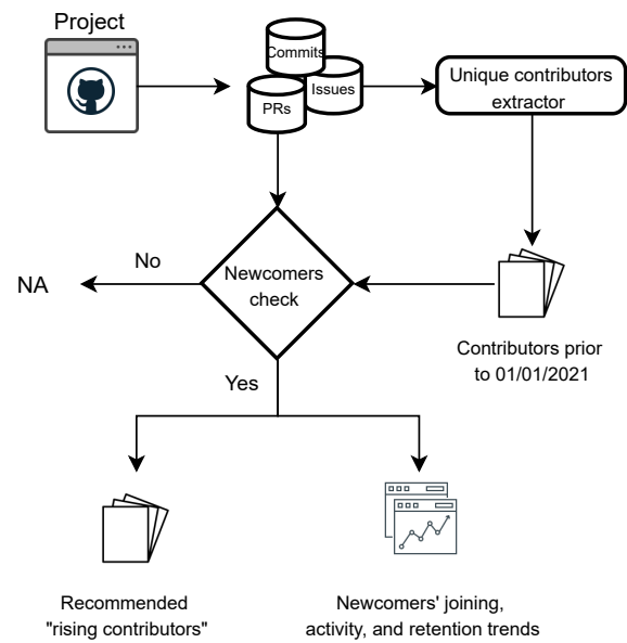
Figure 1: Implementation approach of the community growth recommendation: "rising contributor".
