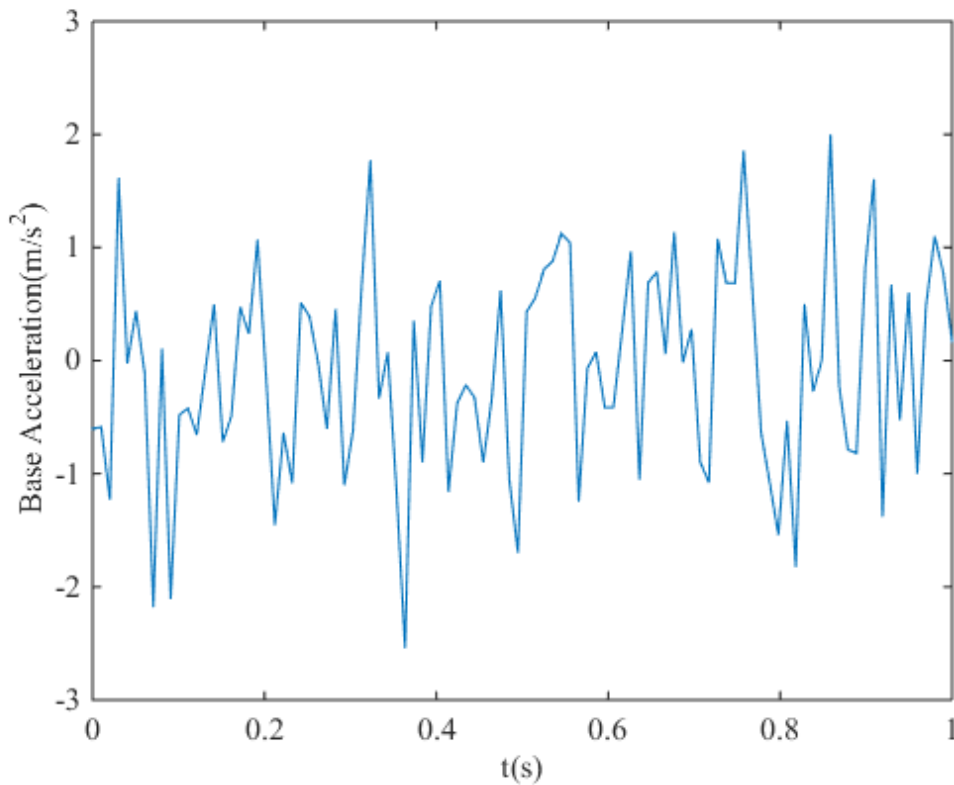
Figure 6 Base excitation
