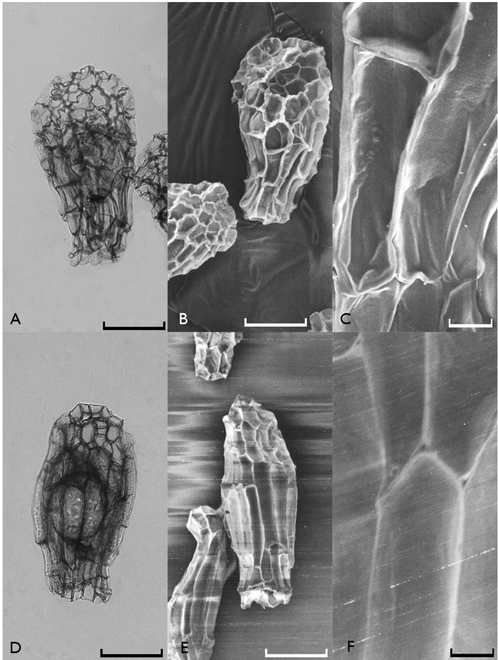
Figure 3. Light microscope (A, D) and scanning electron microscope (B, C, E, F) photographs of Orchis mascula subsp. mascula (A, B, C) and O. purpurea subsp. purpurea (D, E, F) seeds. Scale bars: 0.1 mm (A, B, D, E) and 0.01 mm (C, F).
