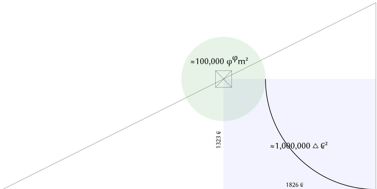
Figure 40: Silver ratio and \varphi^\varphi
