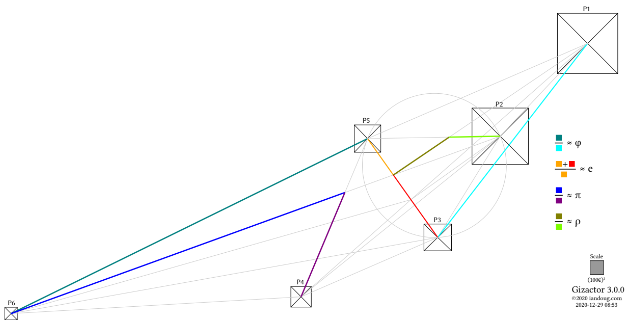
Figure 36: \pi , \phi , e and \rho .
