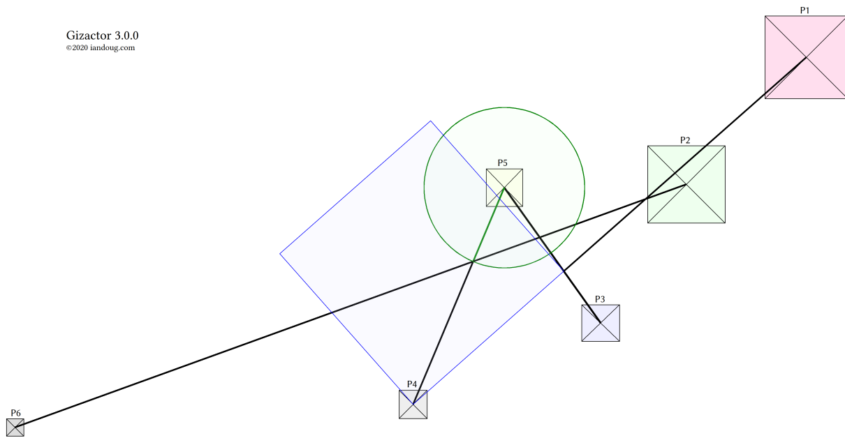
Figure 46: Doubling the area, circle to square.
