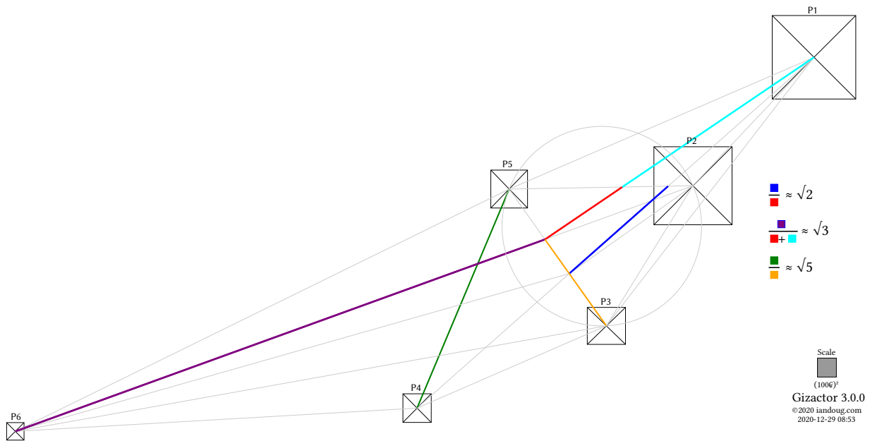
Figure 35: Square roots of the first three primes.
