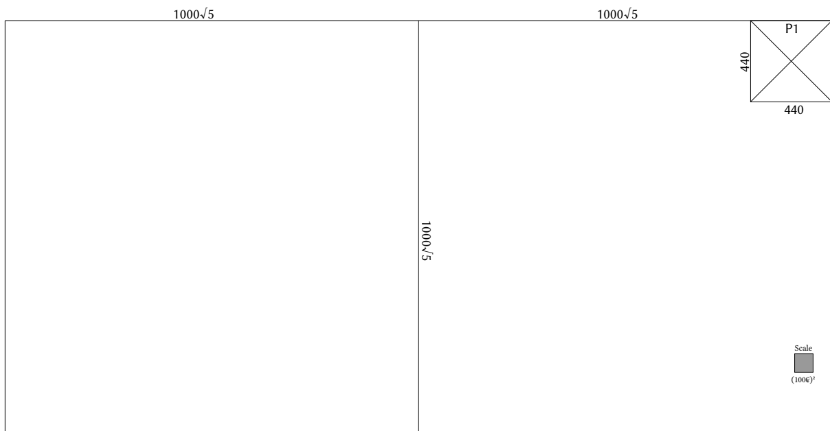
Figure 7: The Giza plan outer bounding rectangle
