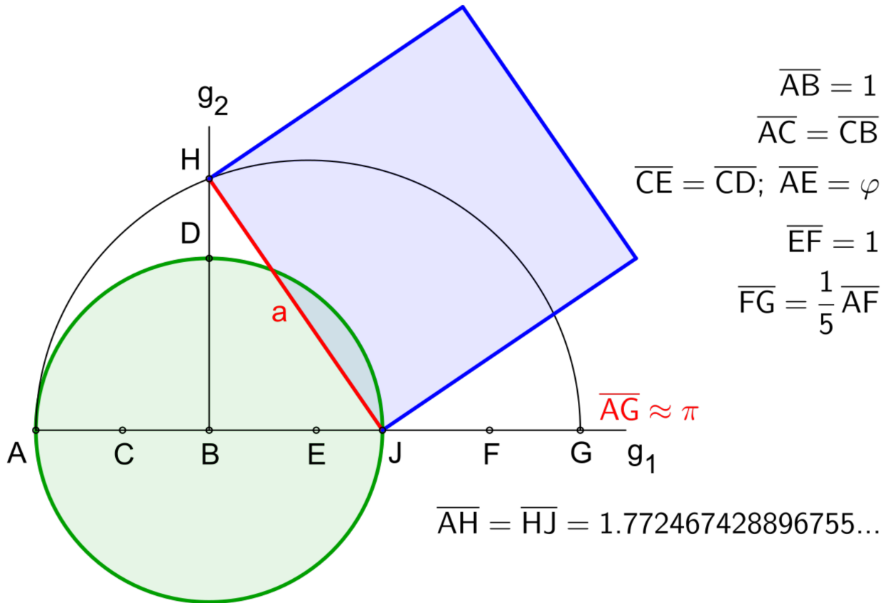
Figure 41: Squaring the circle, Robert Dixon "Golden Ratio" method.
