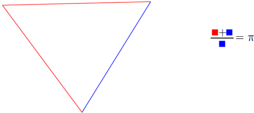
Figure 20: The \pi triangle.
