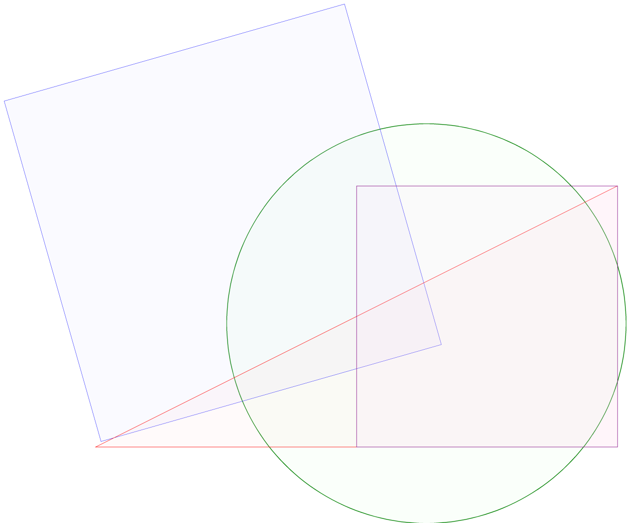
Figure 45: The search for equality.
