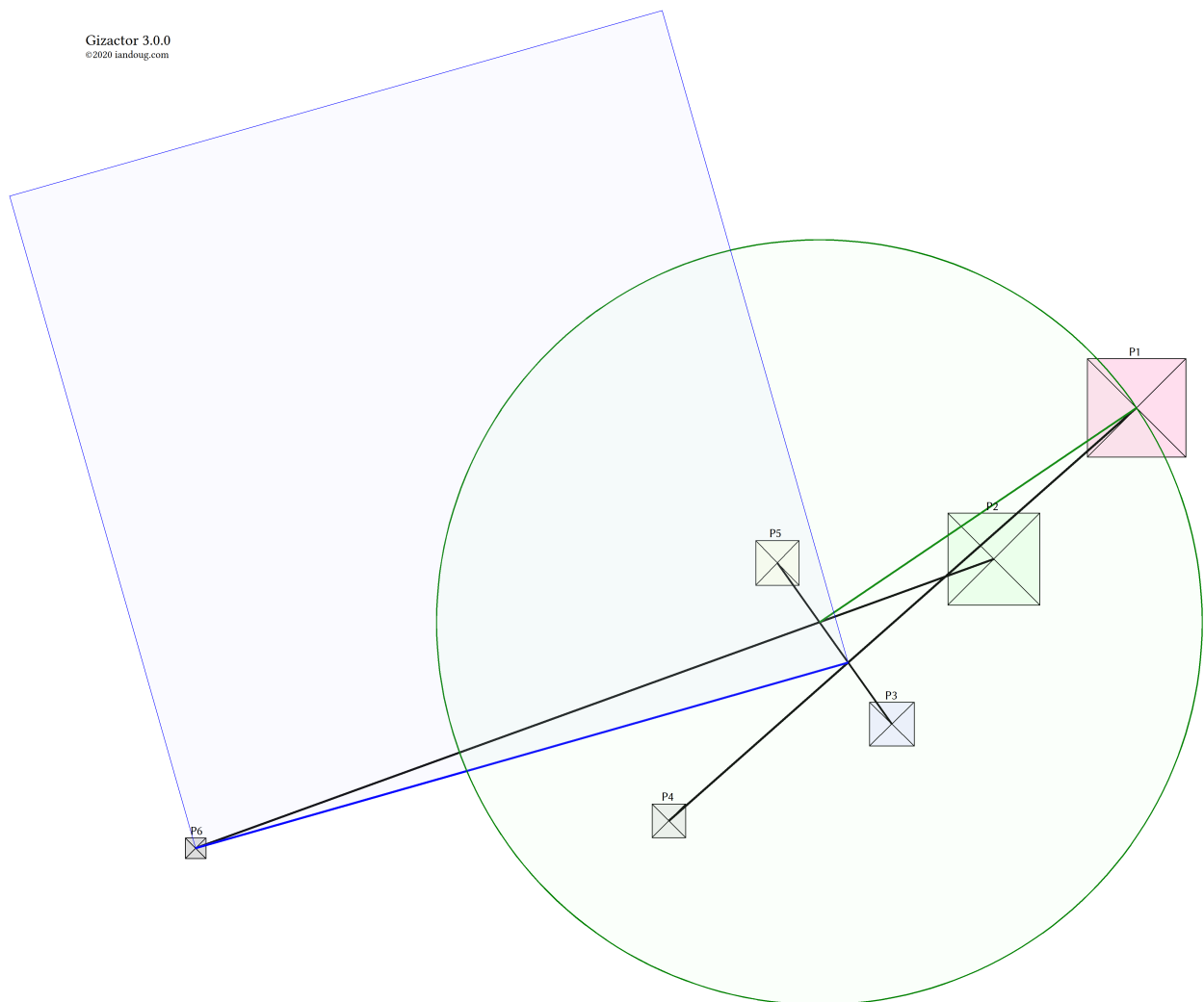
Figure 44: Squaring the circle, Texas style, where everything is bigger.
