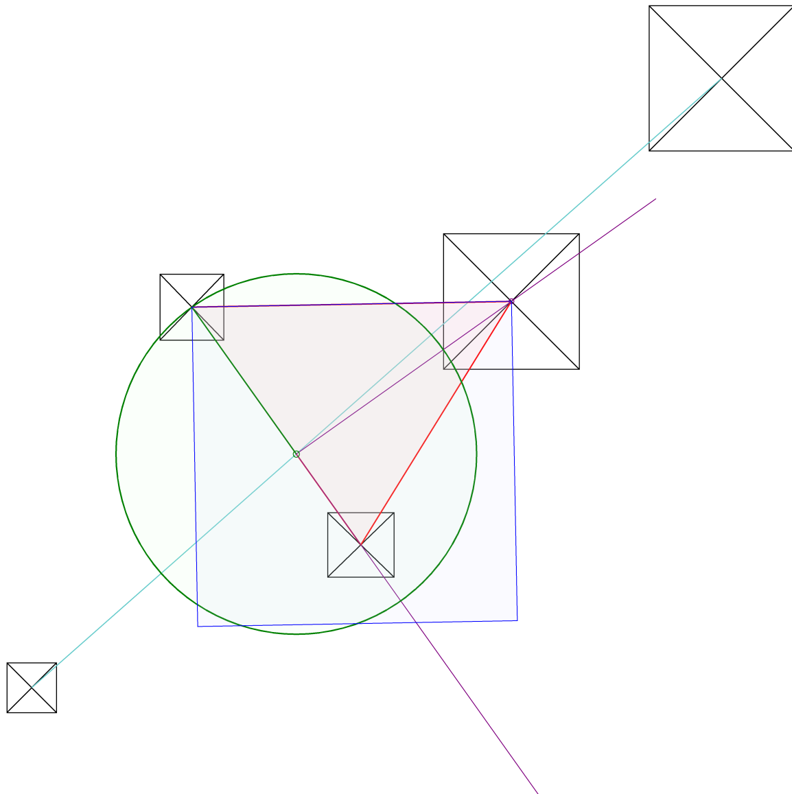
Figure 43: Squaring the circle, Giza style.
