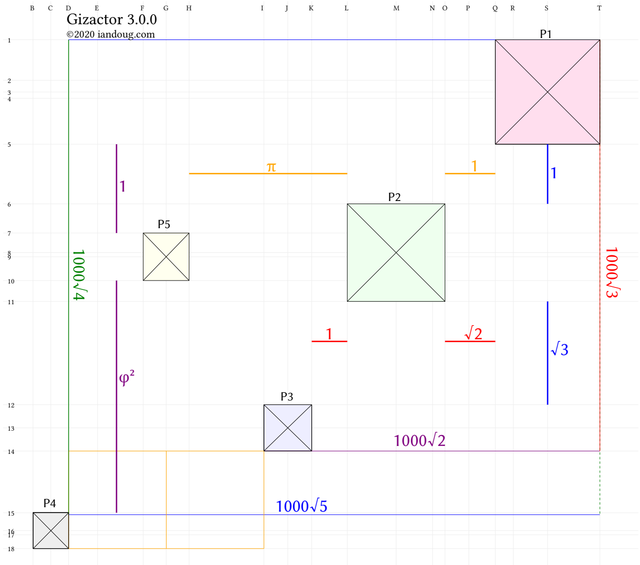
Figure 16: Master plan for laying out Giza right side.
