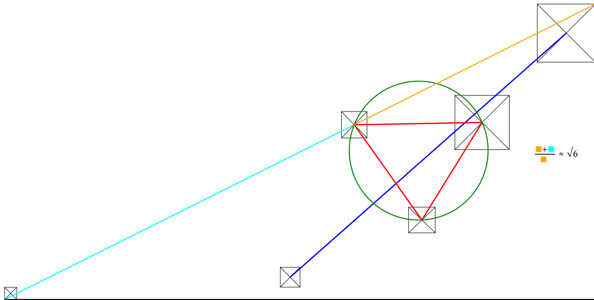
Figure 38: How P5 divides the diagonal.
