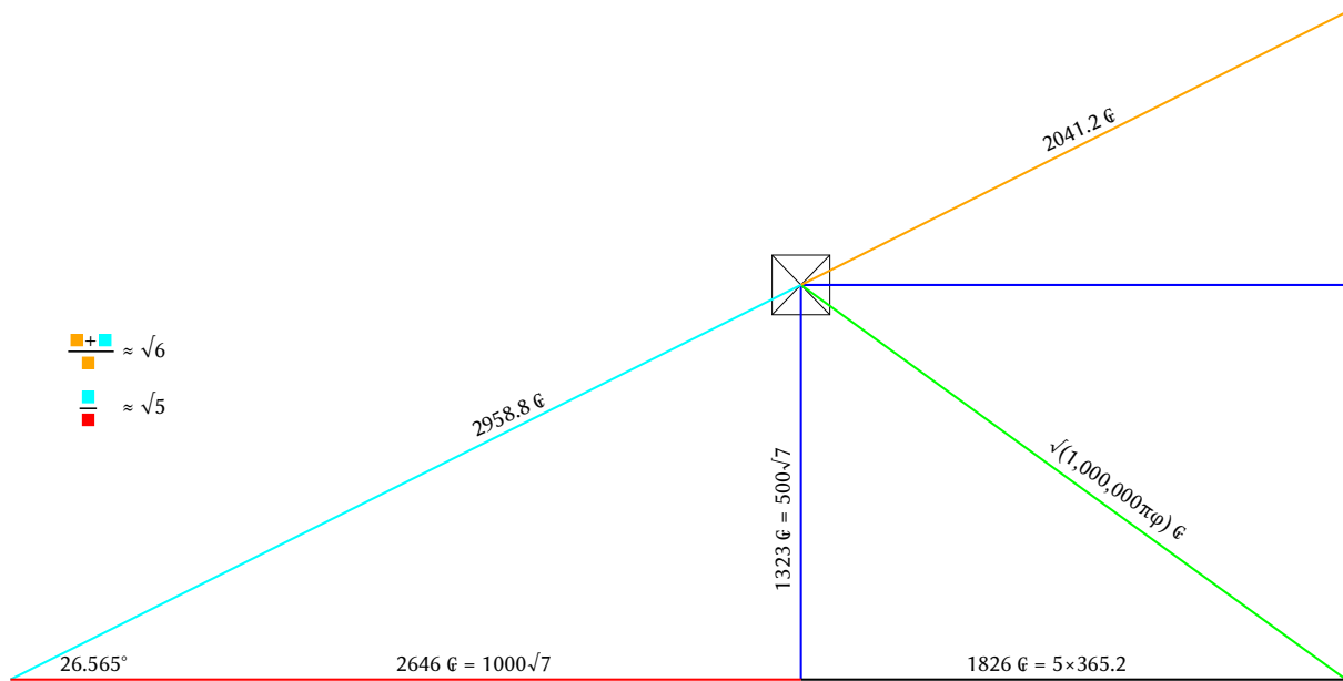
Figure 39: From \sqrt{6} to \sqrt{7} , \sqrt{5} and a year.
