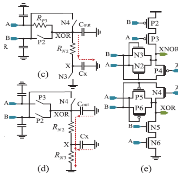
Fig.2. (c) RC model of proposed XOR for AB = 10 . (d) RC model of proposed XOR for AB = 11 . (e) Modified XOR-XNOR gate.
