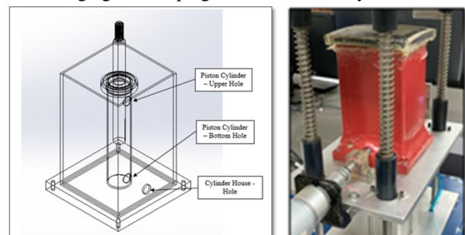
Fig2: Variable damper Design
