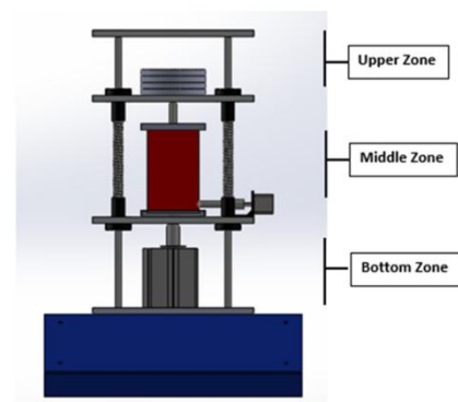
Fig1:CAD Model of the suspension system
