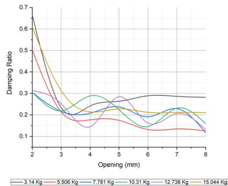
Fig7. Damping ratio variations at constant weights with the variable openings for spring K1
