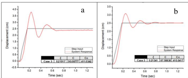
Fig6. Experimental and calculated response for case3
