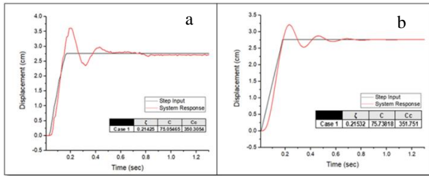
Fig4. Experimental and calculated response for case1
