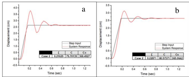
Fig5. Experimental and calculated response for case2
