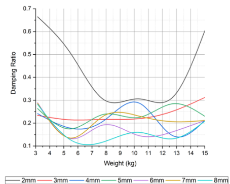
Fig8. Damping ratio variations at a constant opening with the variable weights for spring K1
