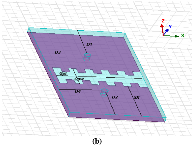
Figure.1 Design of 2 port antenna (a) 3-D view of model (b) Ground plane with substrate
