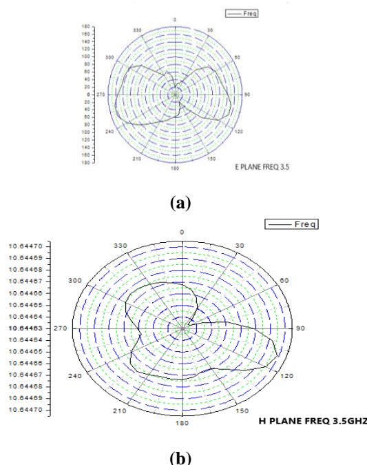
Figure 6 The simulated and measured radiation patterns of the proposed MIMO antenna in (b) the x-y (H-plane) and (a) y-z (E-plane) planes at 3.5GHz
