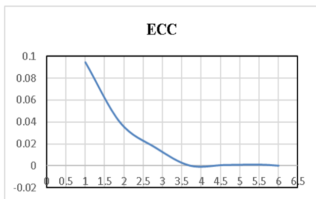
Figure 5 envelope correlation coefficient of proposed model
