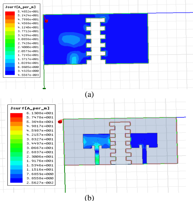
Figure 7 Current distribution of ground plane when both ports are active(a) and the current distribution when one port is active(b)
