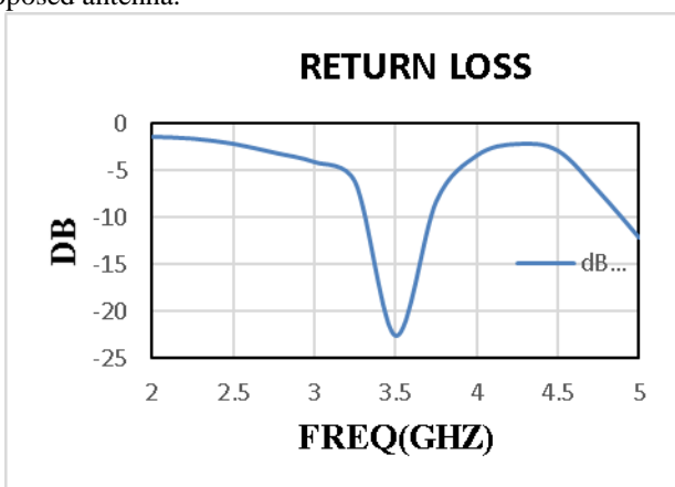
Figure 4 return loss
