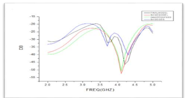
Figure 3 isolation results for different parameters Return loss
