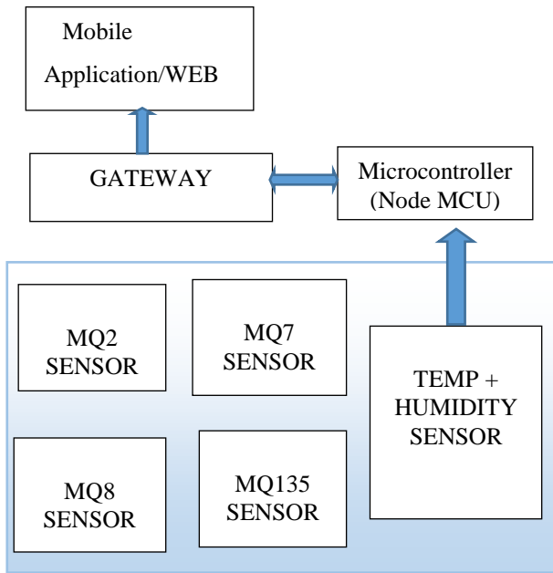
Figure 4.1 Proposed Architecture
