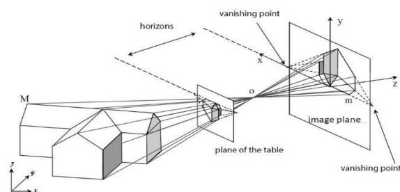
Fig. 1 Perspective image formation.
