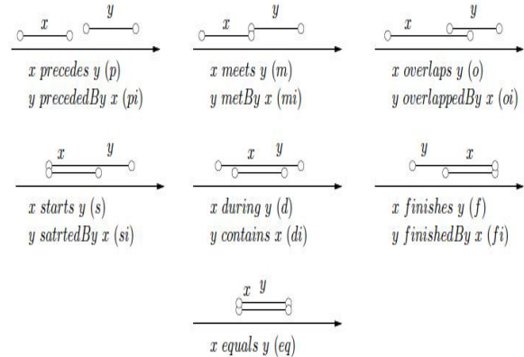
Fig. 3. Allen's Relations.
