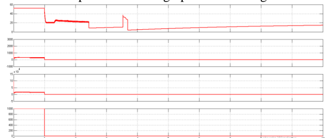
Fig. 11. PV voltage and power for different irradiances
