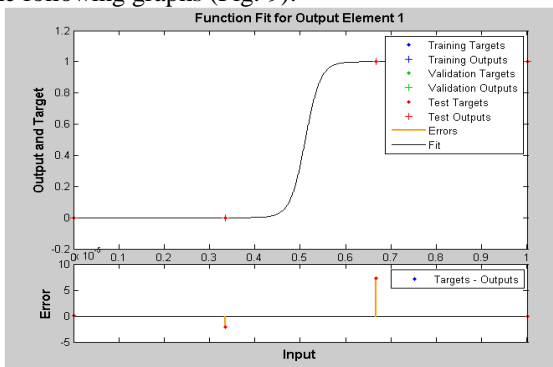
Fig. 9. Fitting curves from neural network training
