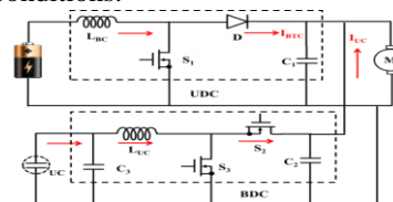
Fig. 5. Converter Mode-III circuit diagram with HESS.
