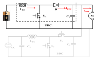
Fig. 4. Converter Mode-II circuit diagram with HESS.
