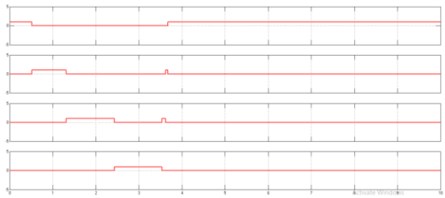
Fig. 13. Modes of Operation Control Waveforms
