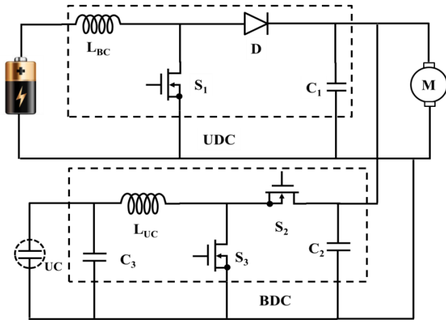
Fig. 2. Circuit Diagram of Converter. (Unidirectional and Bi Directional Converter connected across BLDC motor)
