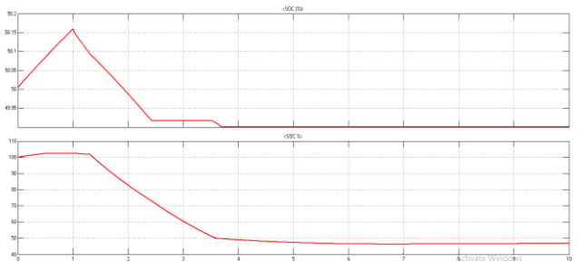
Fig. 14. %SOC of the Battery and UltraCapacitor
