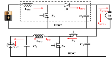
Fig. 3. Converter Mode-I circuit diagram with HESS.
