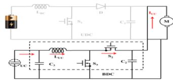
Fig. 6. Converter Mode-IV circuit diagram with HESS.
