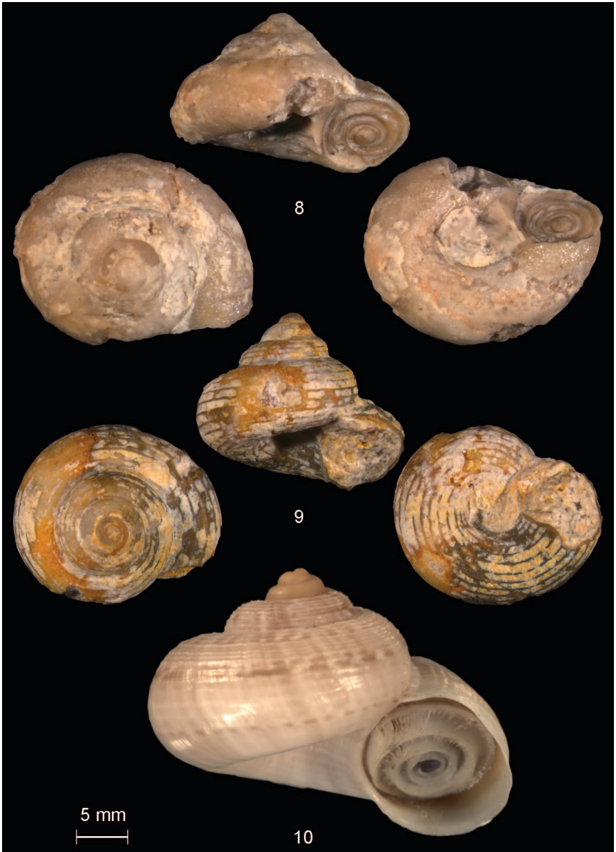
Figs. 8–10: Cyclotopsis praecursor sp. nov. Fig. 8: Thaytiniti , holotype NMBE 5018970 in frontal, apical and ventral view; Fig. 9: Wadi Darbat, paratype NMBE 5018974 in frontal, apical and ventral view; Fig. 10: Cyclotopsis semistriatum (SOWERBY, 1843), syntype NHMUK 20030591, India, Poona.
