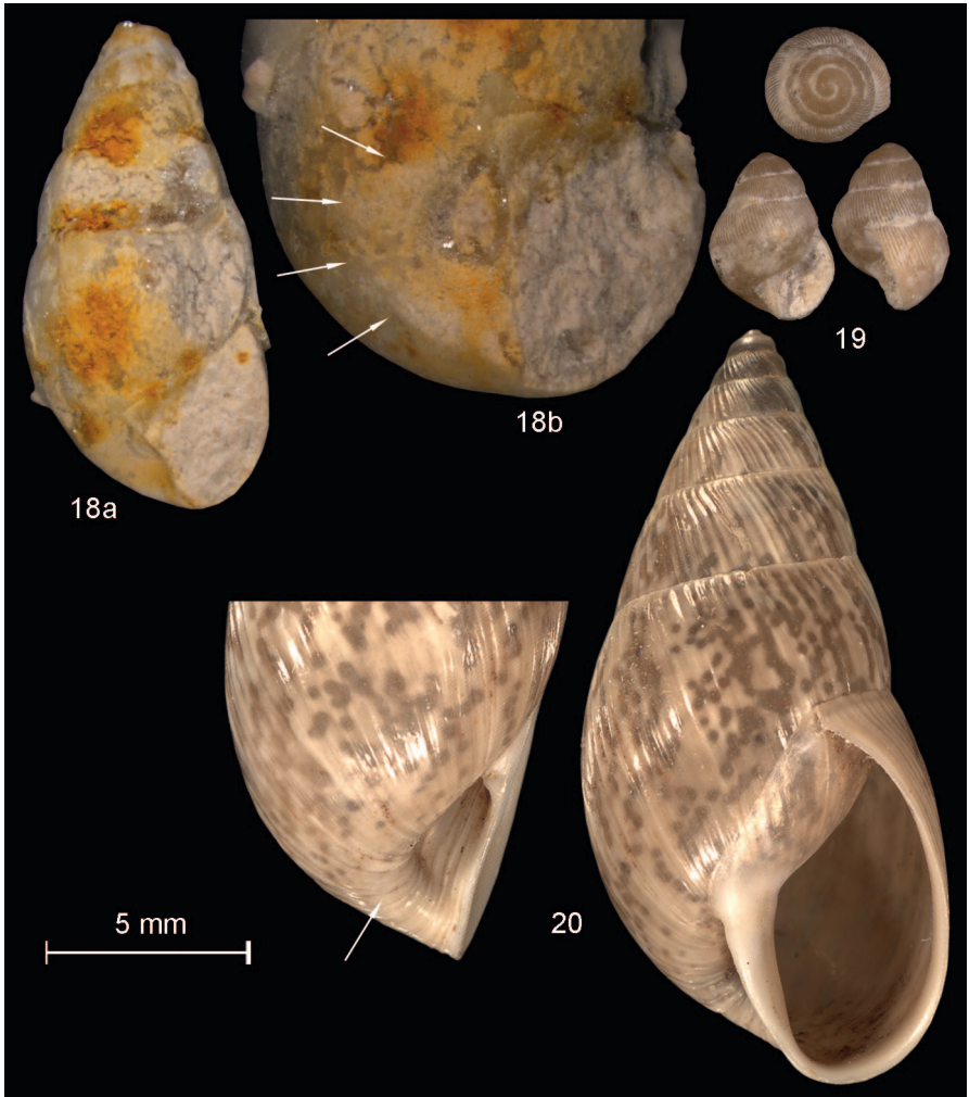
Figs. 18–20: Species of Cerastidae. Fig. 18a: Cerastus praeinsularis sp. nov., Wadi Darbat, holotype NMBE 5018986 in frontal view. Fig. 18b: ditto, detail of last teleoconch whorls with the periomphalum. Fig. 19: C. praeinsularis sp. nov., only upper whorls preserved, Wadi Darbat, paratype NMBE 5019050. Fig. 20: Achatinelloides hadibuensis , Yemen, Soqatra Isl., Wadi Ayhaft, leg. K. van Damme. Details not to scale.
