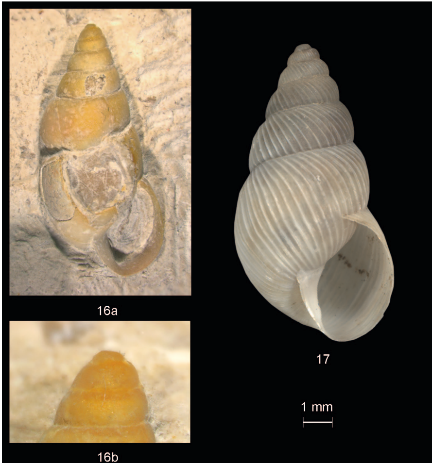
Figs. 16–17: Species of Cerastidae. Fig. 16a: Cerastus pseudoena sp. nov., Wadi Darbat, holotype NMBE 5018985 in frontal view. Fig. 16b: ditto, detail of protoconch and upper teleoconch whorls; detail not to scale. Fig. 17: Cerastus girwanensis CONOLLY, 1941, SMF 311620, Saudi Arabia, Asir province, Wadi al-Sharan S of Bani Sa'ad, 1750 m alt, leg. E. Neubert.
