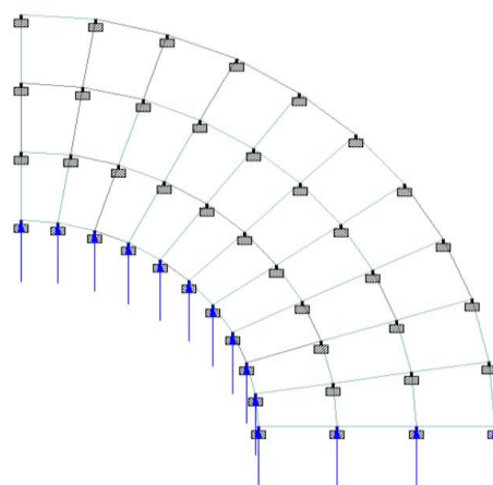
Figure 6. Best orientation of curved structure
