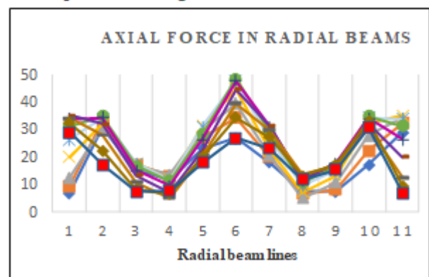
Figure 3. Variation of axial force w.r.t wind load acting inward at different angles
