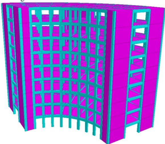
Figure 2. 3-D view of the structure
