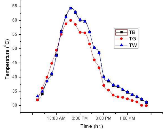
Fig. 4. Temperature of bottom, glass and water on 24 th May 2020
