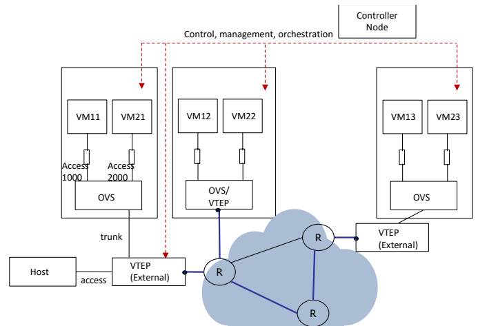
Fig. 3. Example of VXLAN overlay over an IP transport network.
