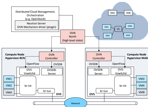
Fig. 4. OVN architecture for the provisioning of virtual overlay networks
